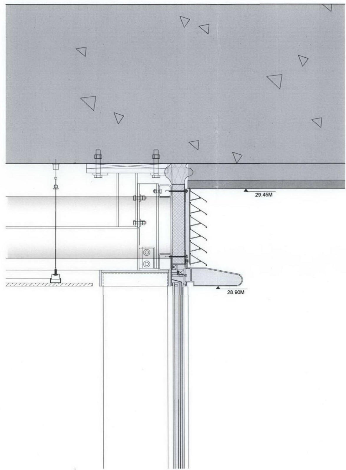
1 EXTERNAL NOSING AND LOUVRE DETAIL SCALE: 1:5 @ A1
