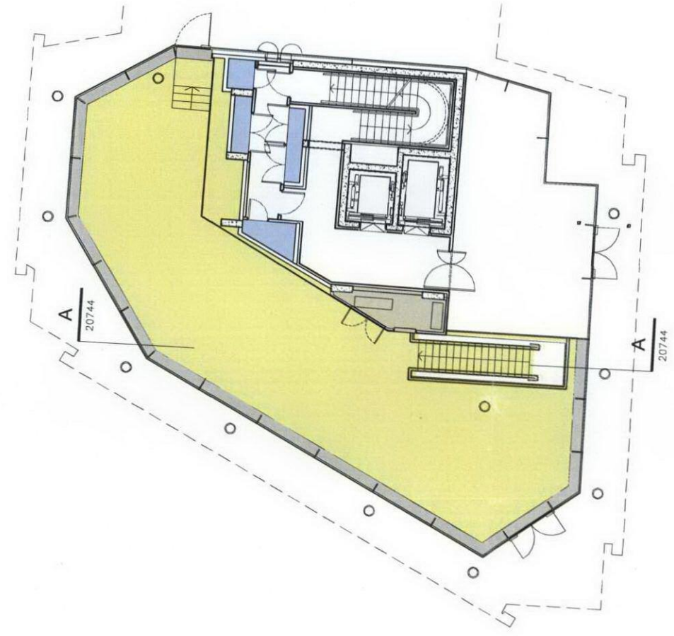
1 RETAIL UNITS 5 PLAN CORE 5 SCALE: 1:100 @ A1
