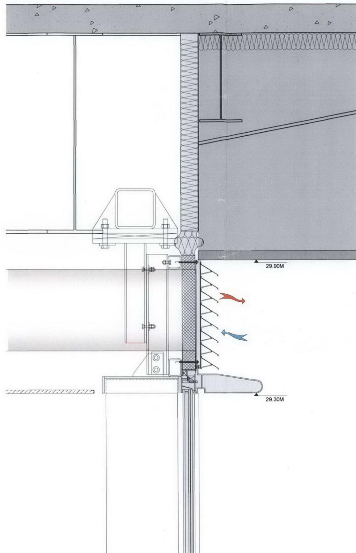
1 EXTERNAL NOSING AND LOUVRE DETAIL SCALE: 1:5 @ A1
