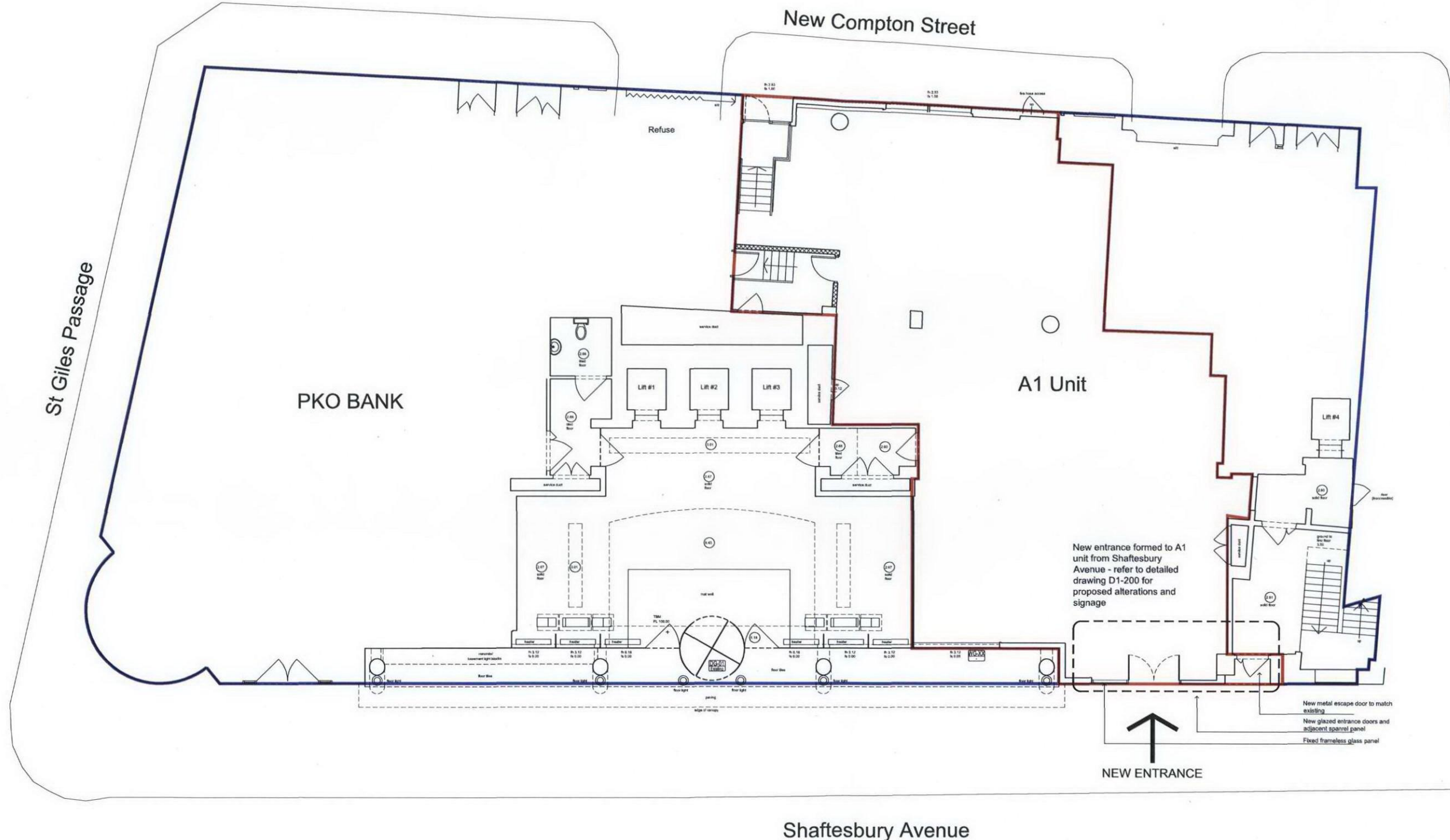
01 GA Floor Plan - Proposed - Ground Floor Plan Scale 1:50
