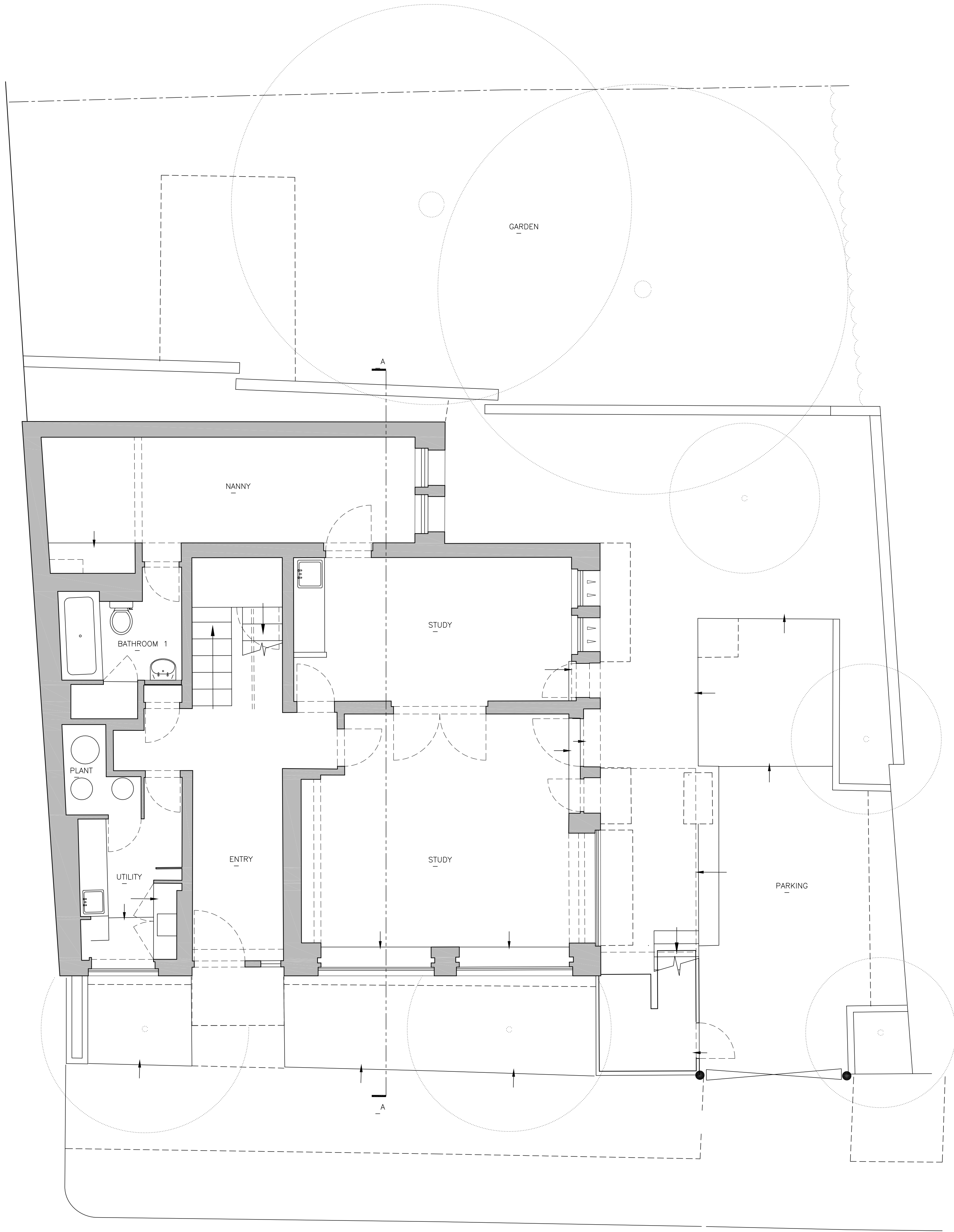
EXISTING GROUND FLOOR
