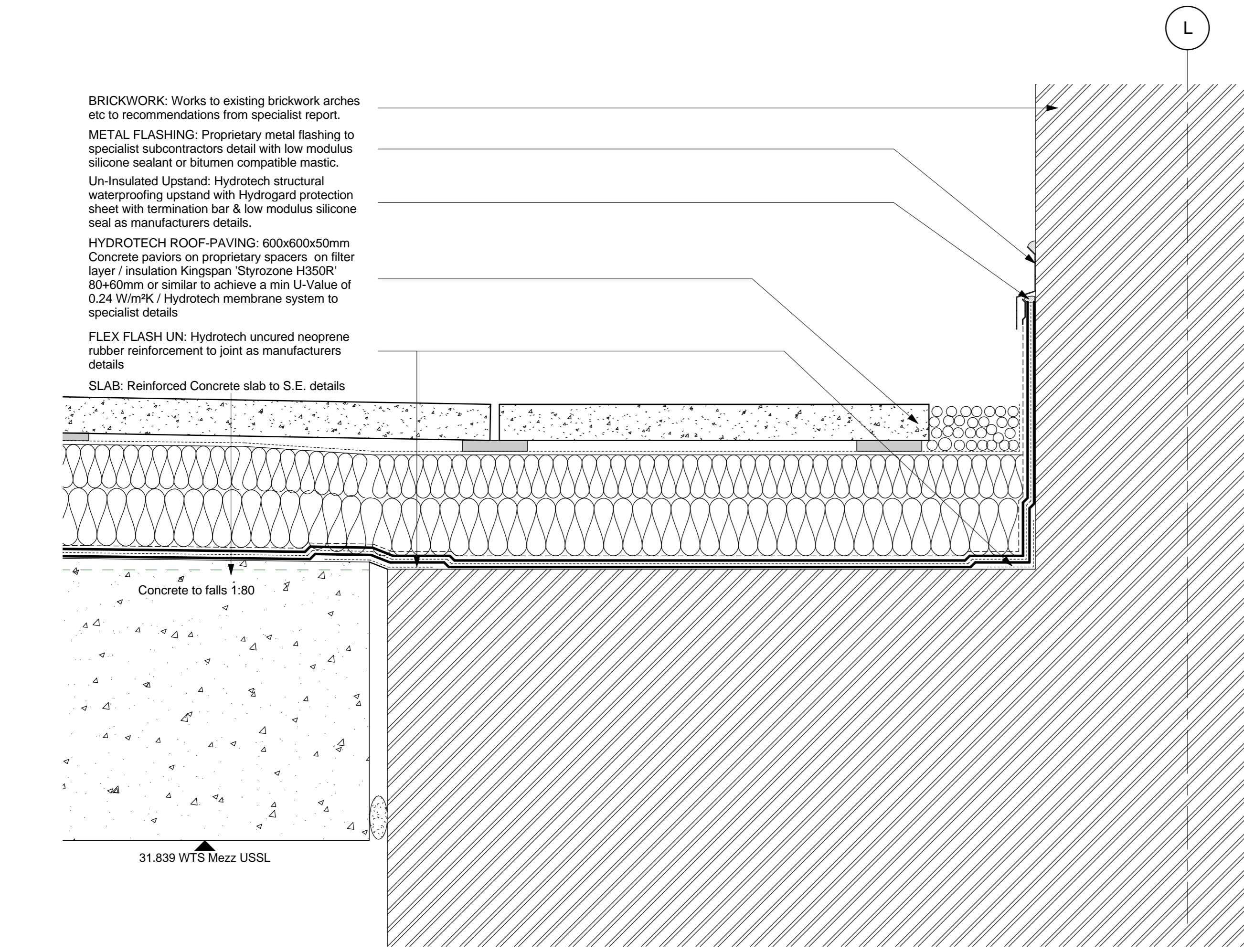
1 WTS - Plant Upstand To Granary 1 : 5
