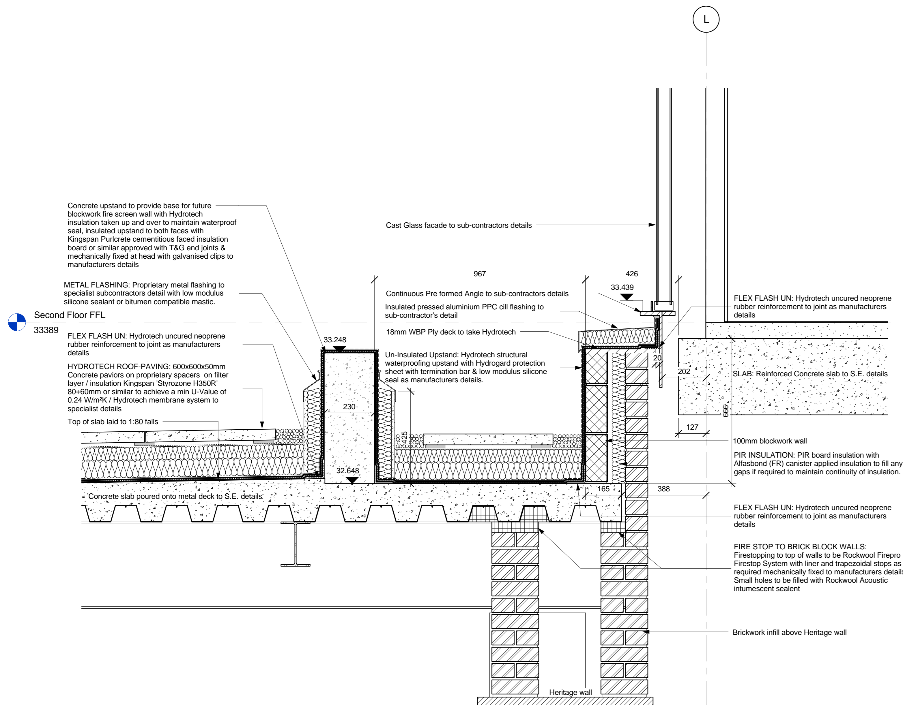
3 WTS-UAL Interface detail 5 1 : 10
