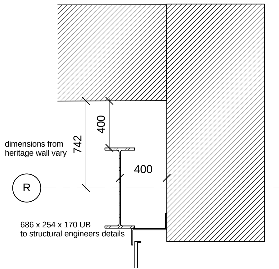
4 WTS - Steel setting out detail 2
