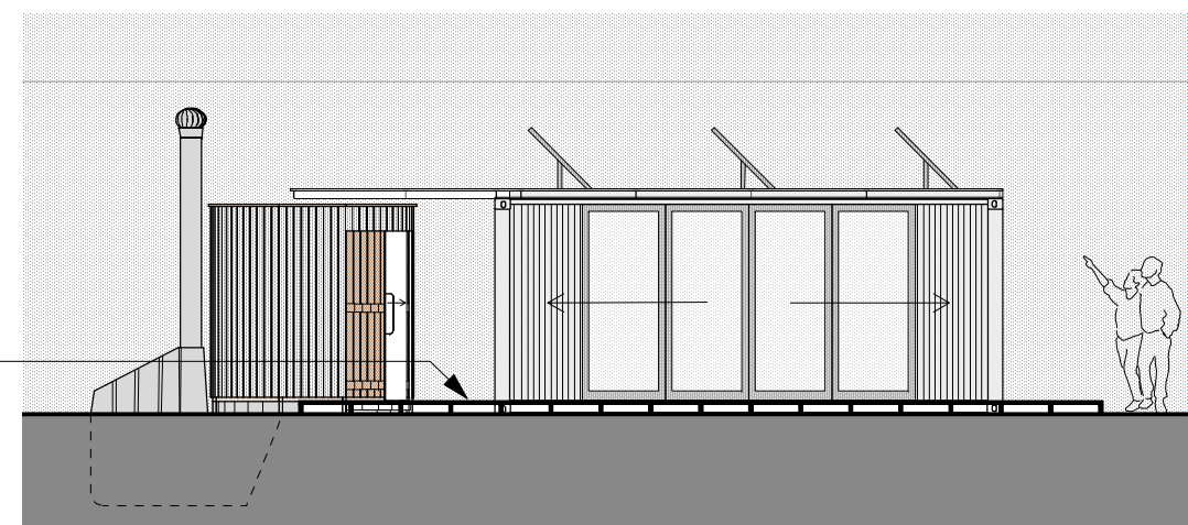
6. Proposed Inner West Elevation
