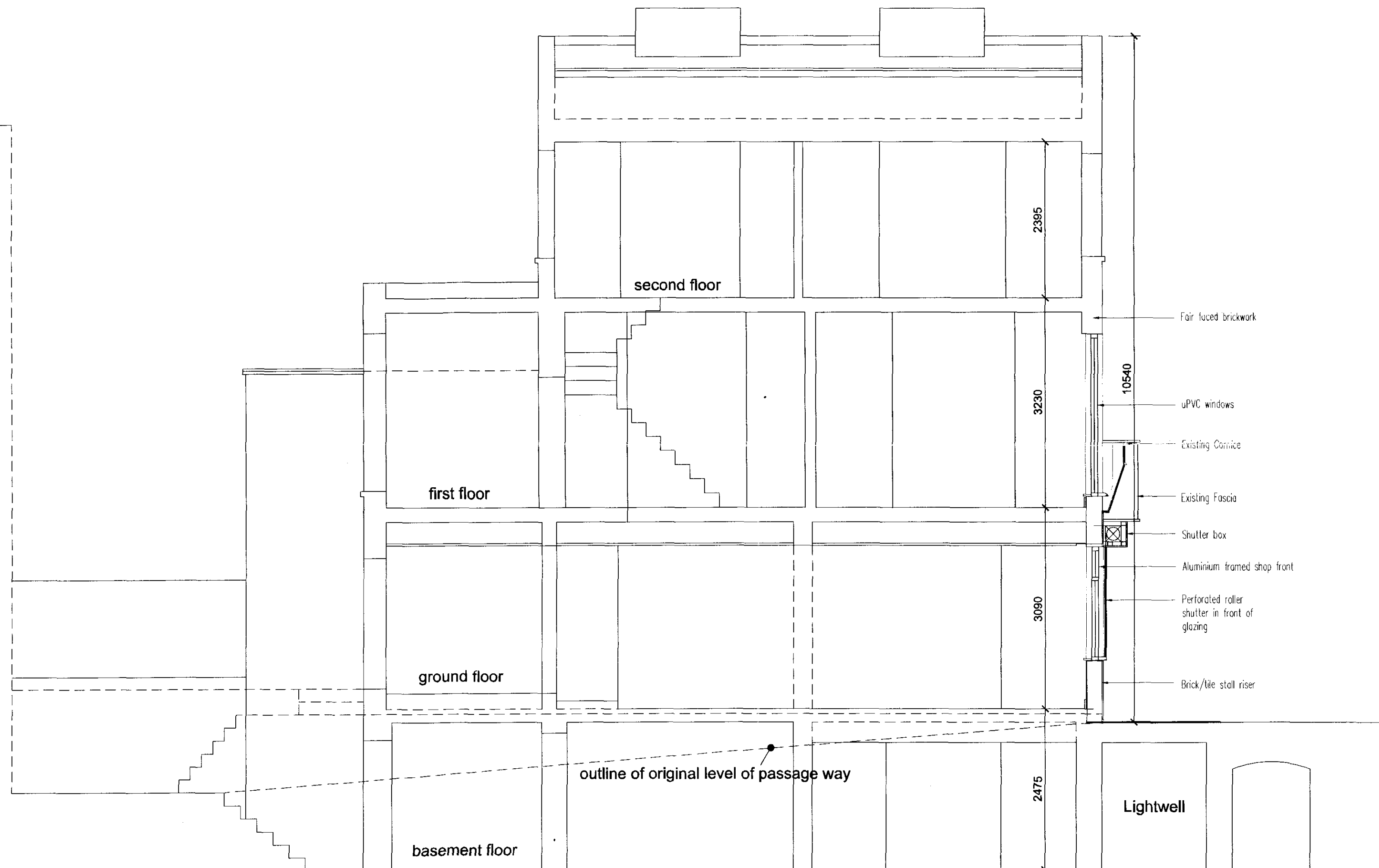
SECTION XX
