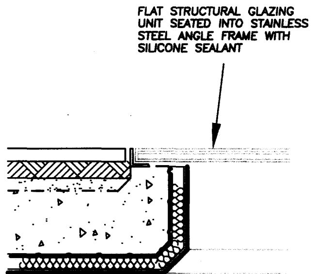
FLUSH STRUCTURAL GLAZING DETAIL
