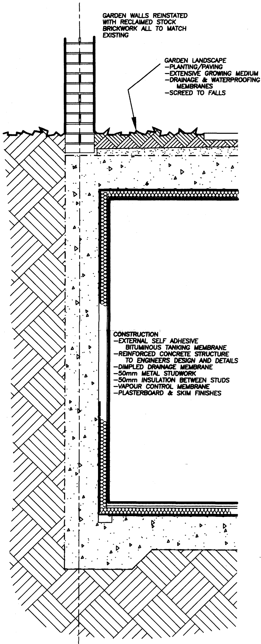
TYPICAL SECTION SHOWING BOUNDARY CONDITION
