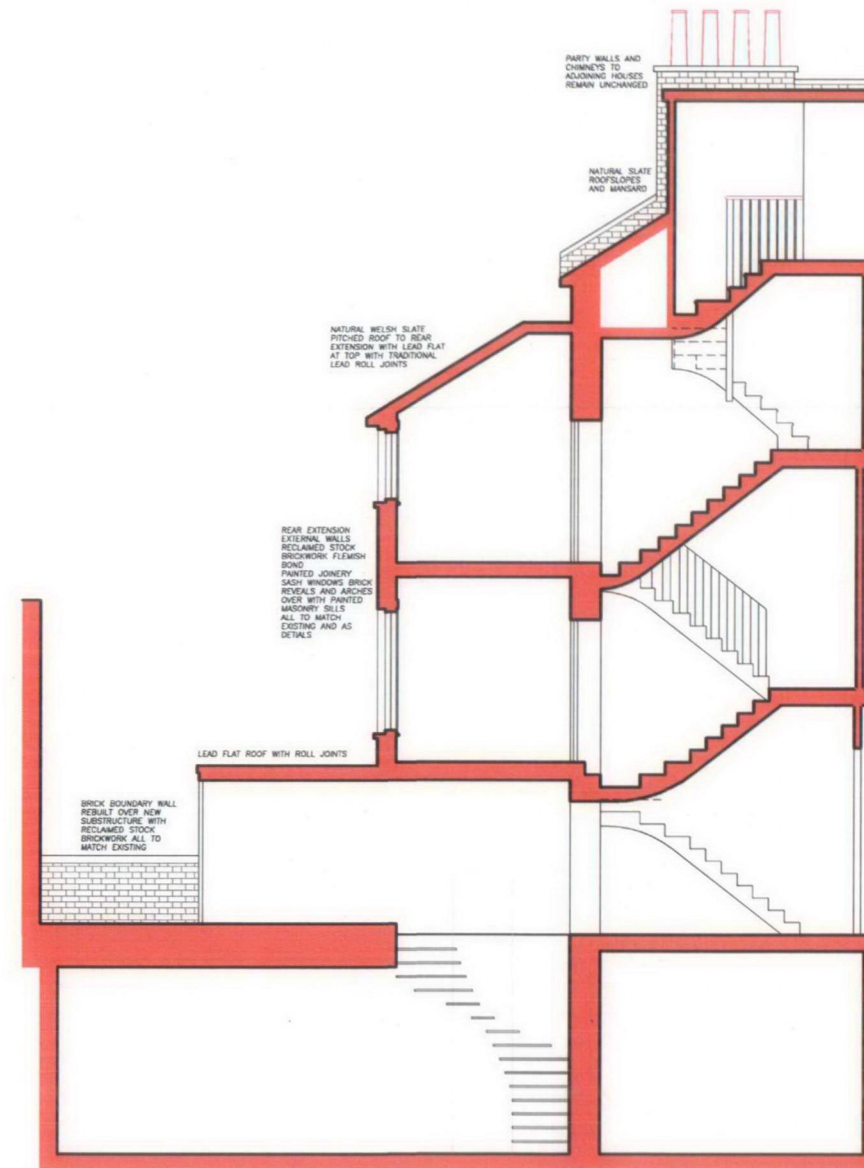
SECTION C
