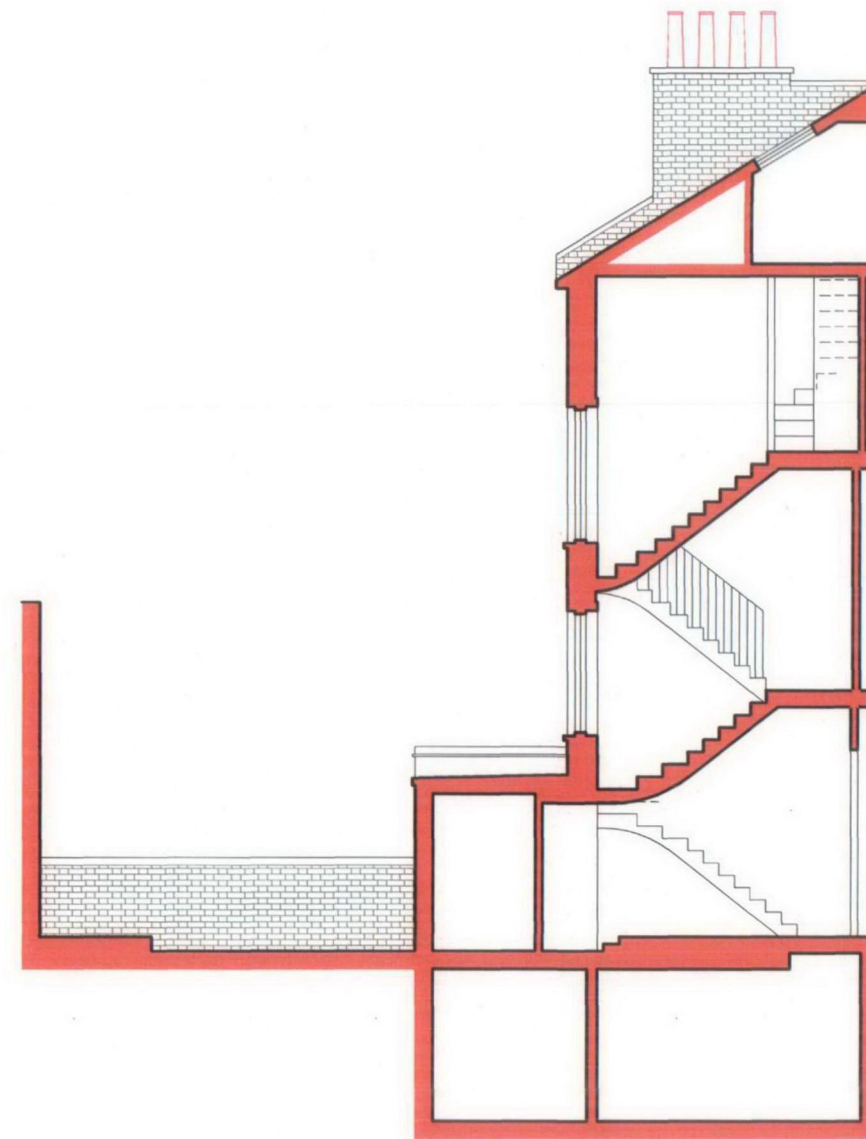
SECTION C
