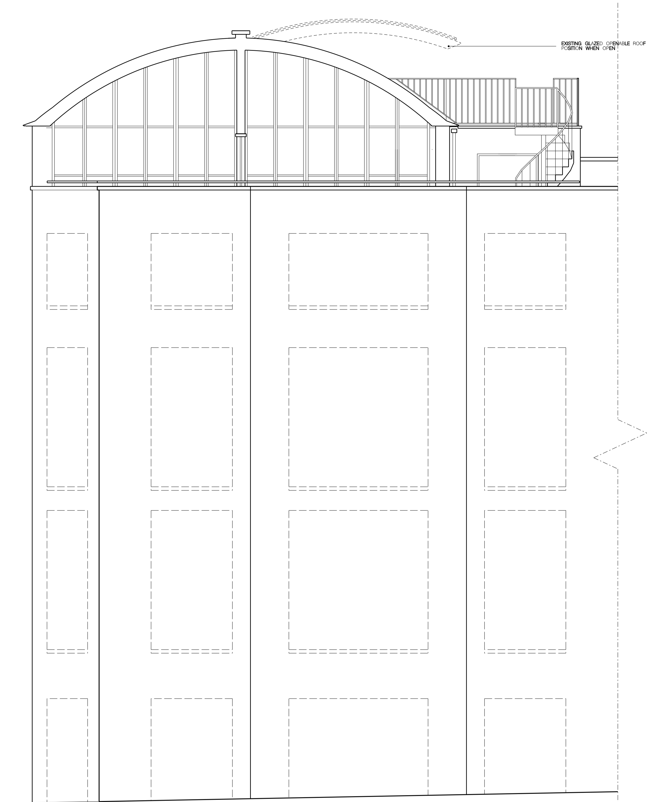
WEST ELEVATION IN CONTEXT INDICATIVE WINDOW LAYOUT AND BUILDING OUTLINE
