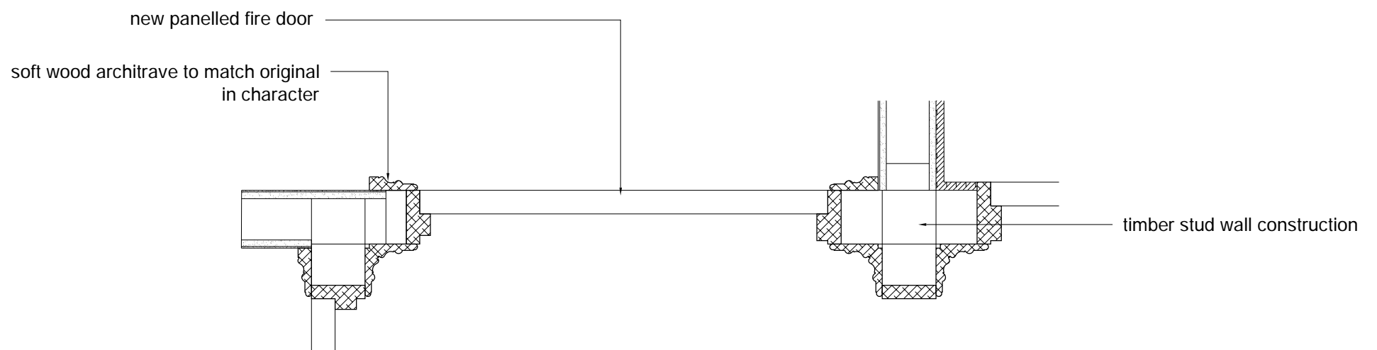
TYPICAL ARCHITRAVE DETAIL
