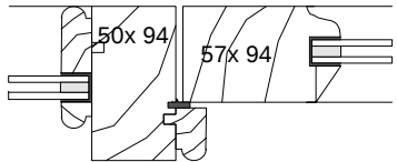
11. door/ Fixed Panel Detail
