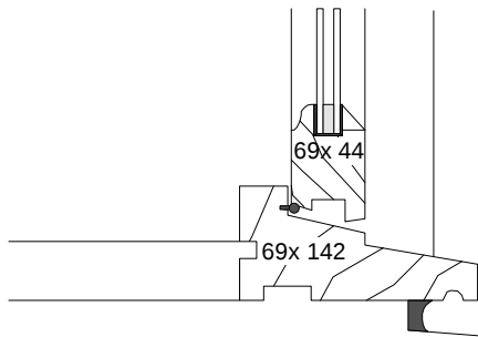
13. Cill Detail
