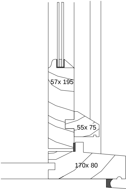
7. Cill Detail
