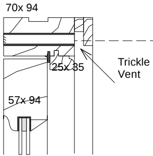
6. Head Detail
