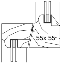
2. Meeting Rail Detail
