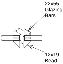
5. Glazing Bar Detail
