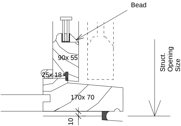
3. Cill Detail
