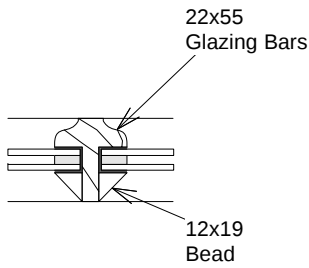
15. Glazing Bar Detail
