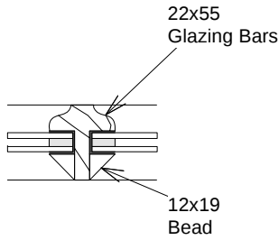
9. Glazing Bar Detail
