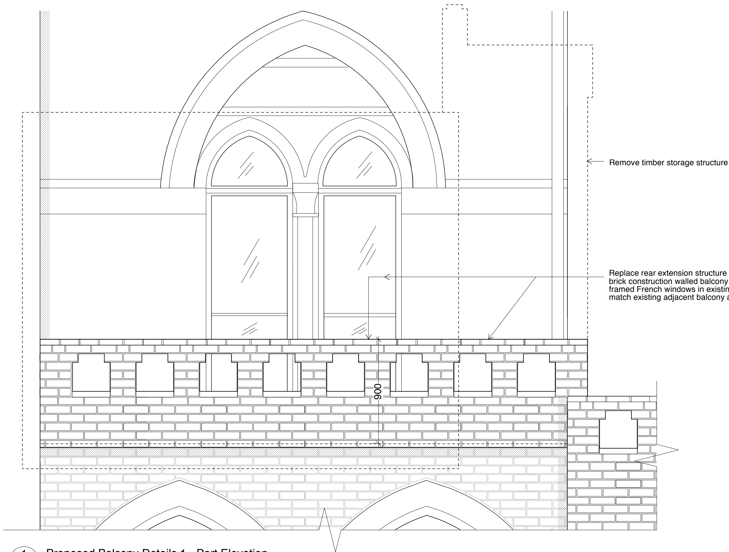
1 Proposed Balcony Details 1 - Part Elevation 150 Scale: 1:20
