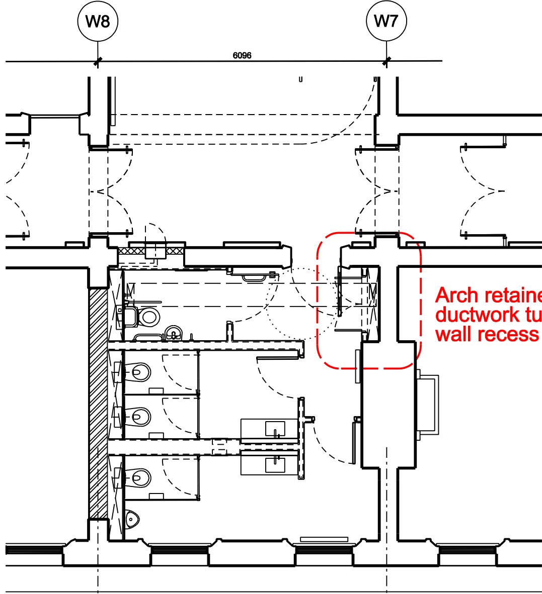
Second floor - Room 2/13
