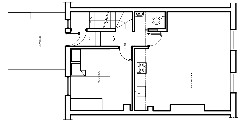
2ND FLOOR AS PROPOSED
