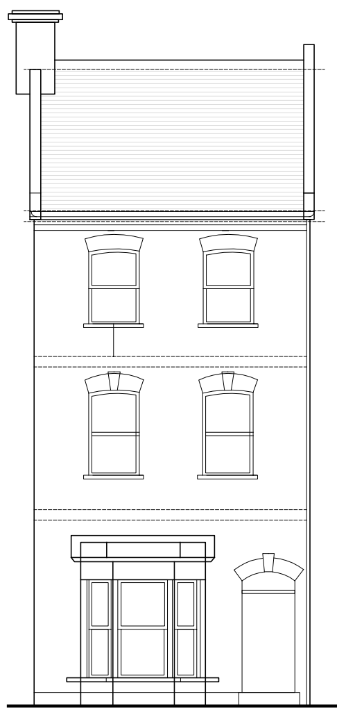
FRONT ELEVATION AS EXISTING
