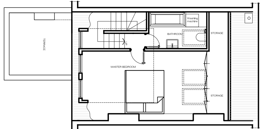
LOFT FLOOR AS PROPOSED
