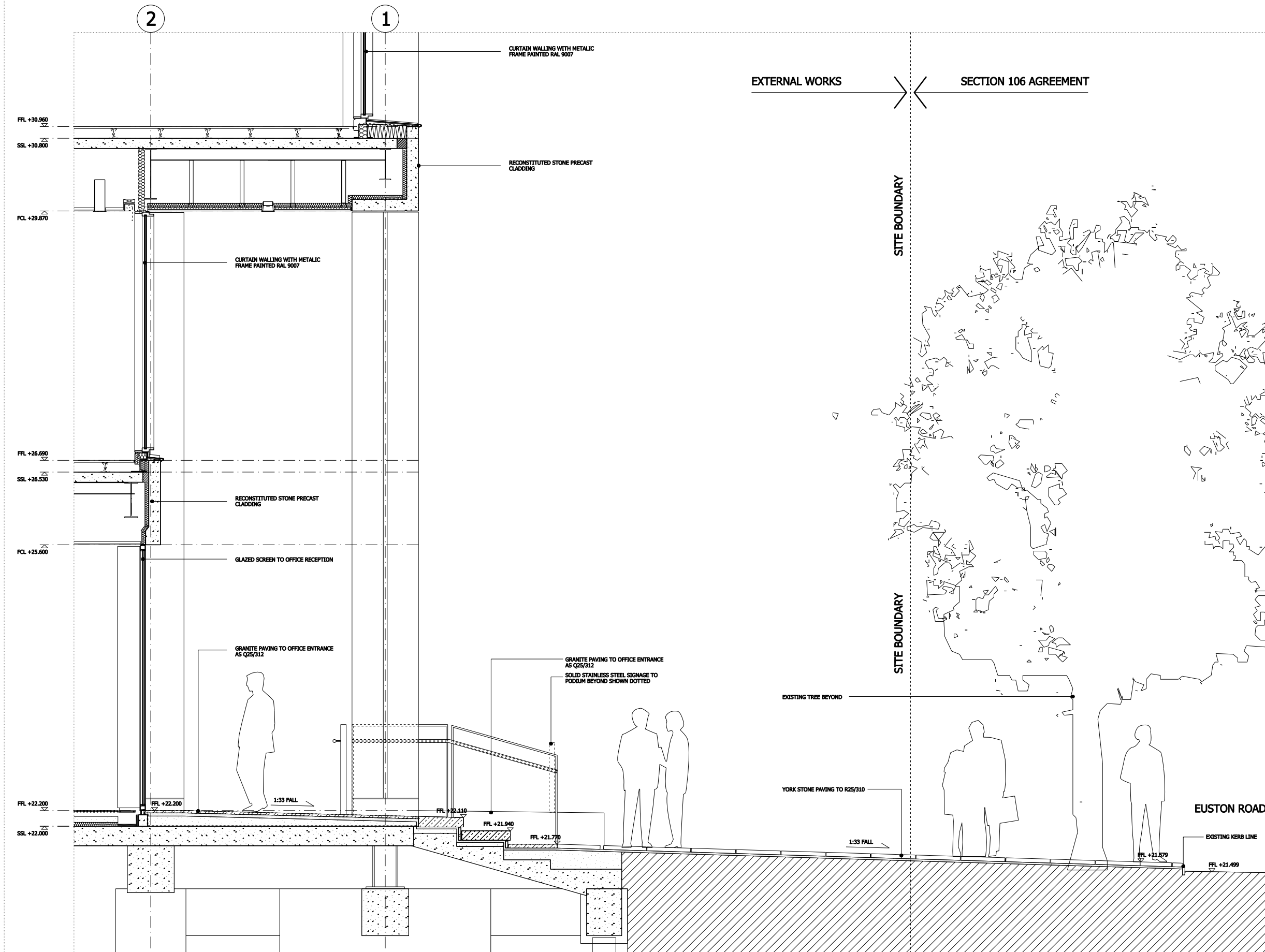
01 SECTION AA - OFFICE ENTRANCE 05070_ExtV_Sect_Block A1 Entry Glazing_01.dgn
