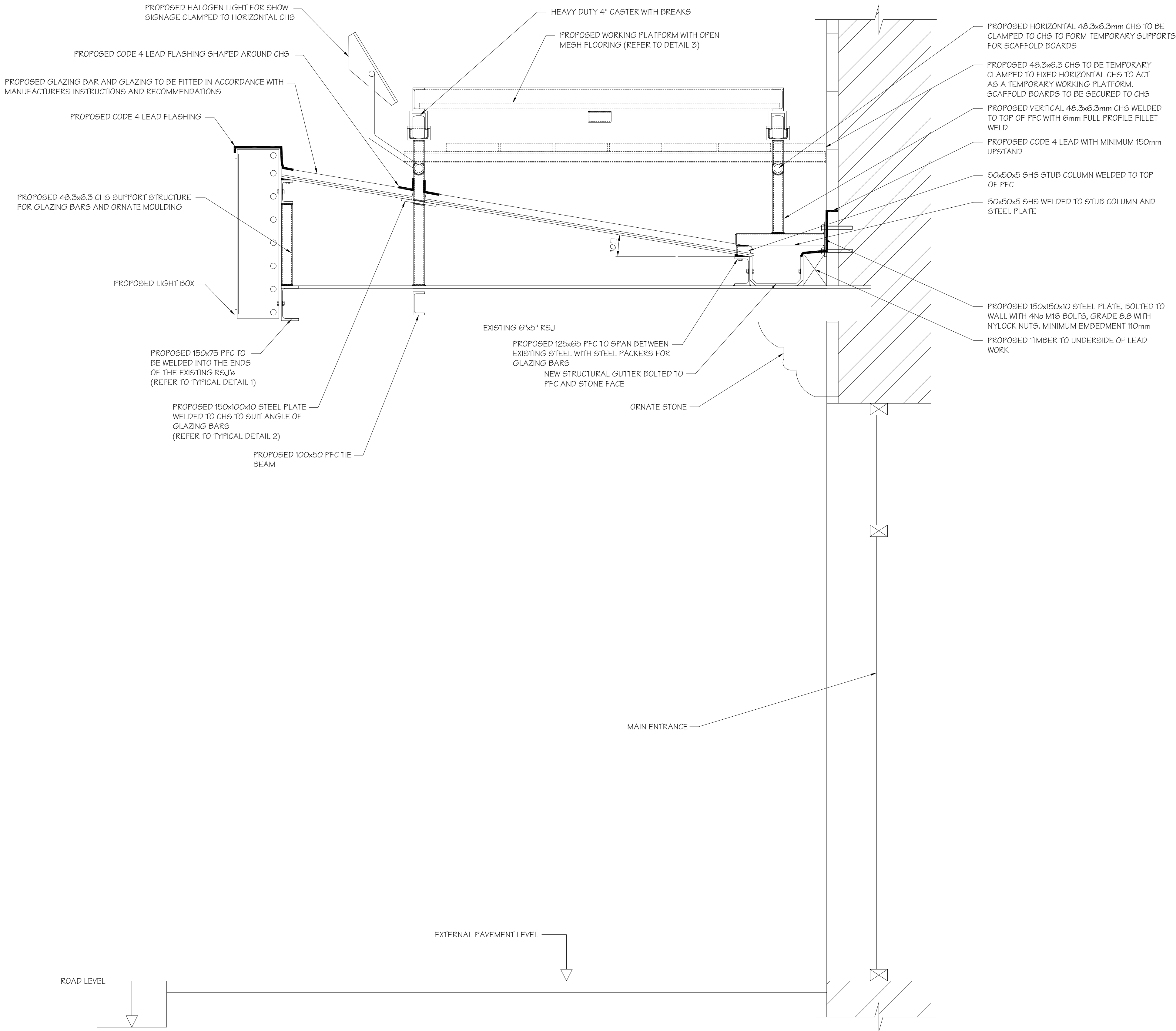
PROPOSED SECTION B-B THROUGH CANOPY OVER THE MAIN ENTRANCE SHOWING LIGHT BOX (SCALE 1:10 AT A1)
