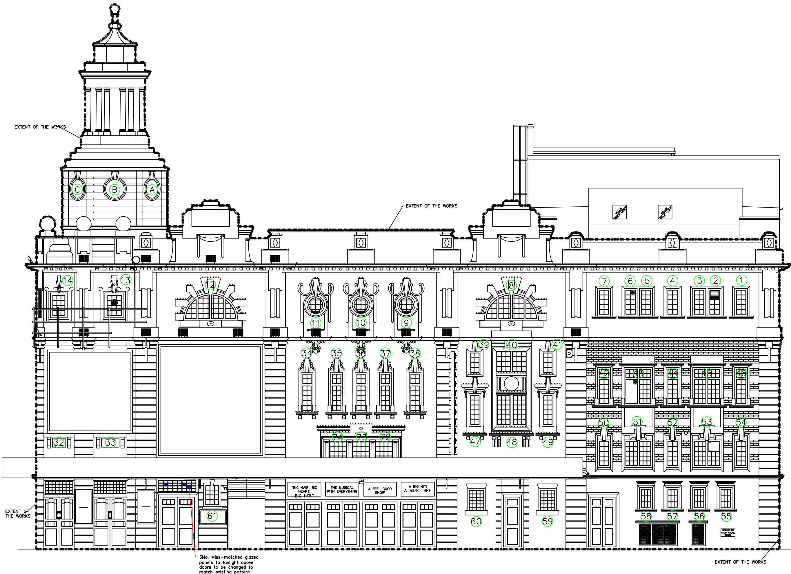
PROPOSED ELEVATION ON HIGH HOLBORN (SCALE 1:50 AT A1)
