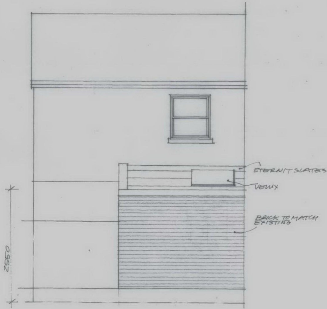
NORTH ELEVATION
