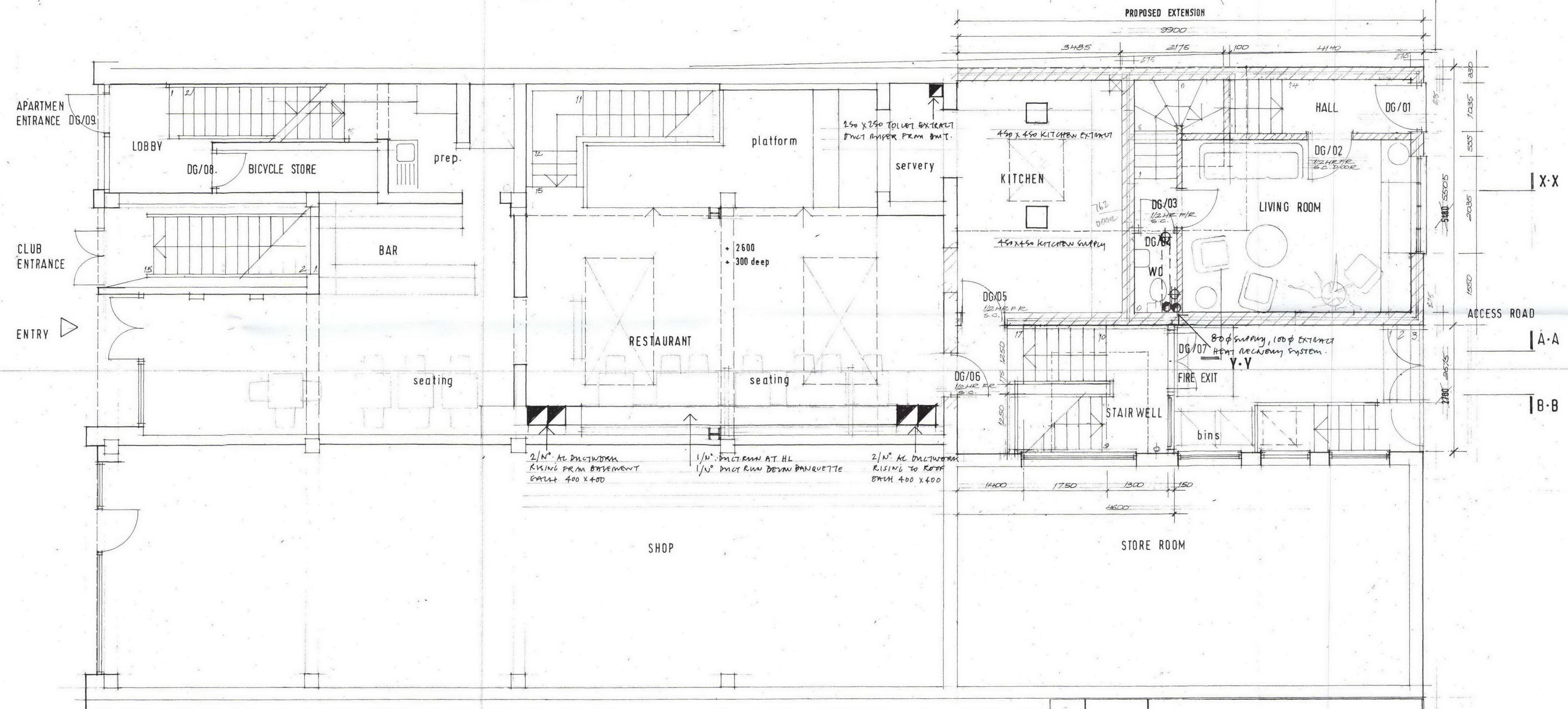
GROUND FLOOR LAYOUT
