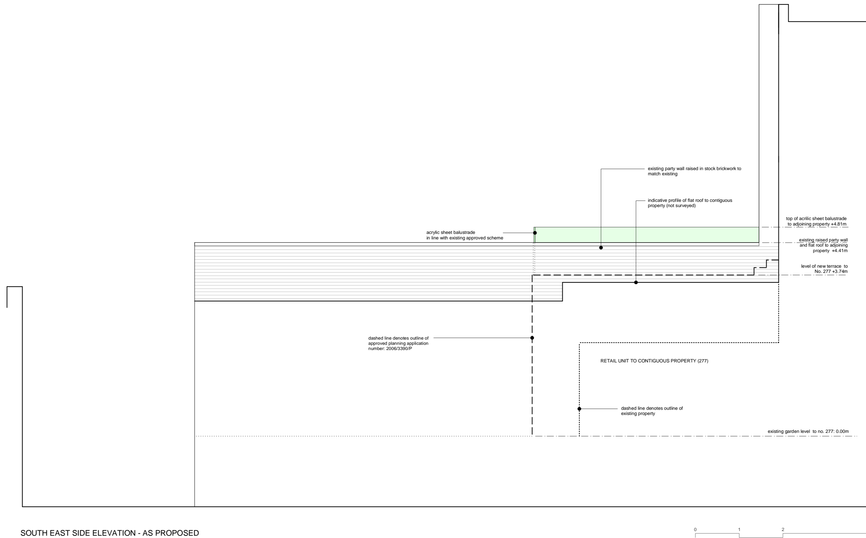
SOUTH EAST SIDE ELEVATION - AS PROPOSED
