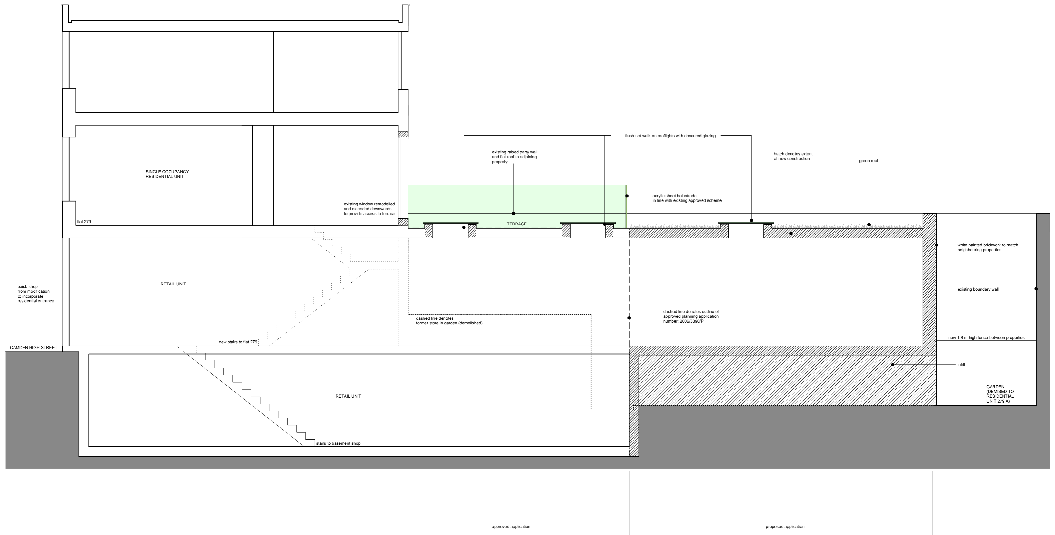
SECTION A-A - AS PROPOSED
