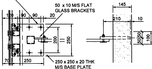
WALL BRACKET DETAIL
