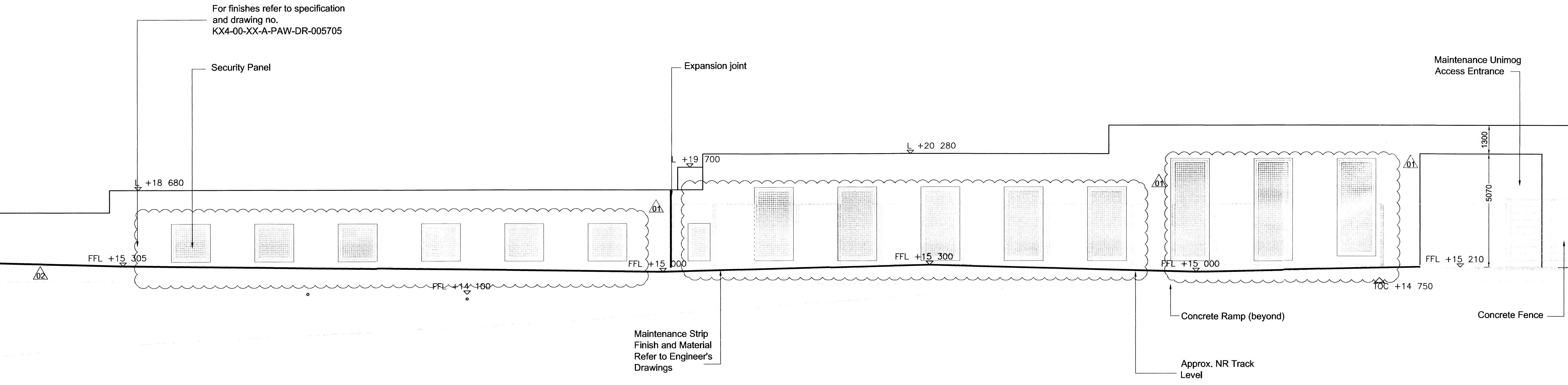
01 ACCESS RAMP ELEVATION (VENTILATION OPENINGS) SCALE 1:100
