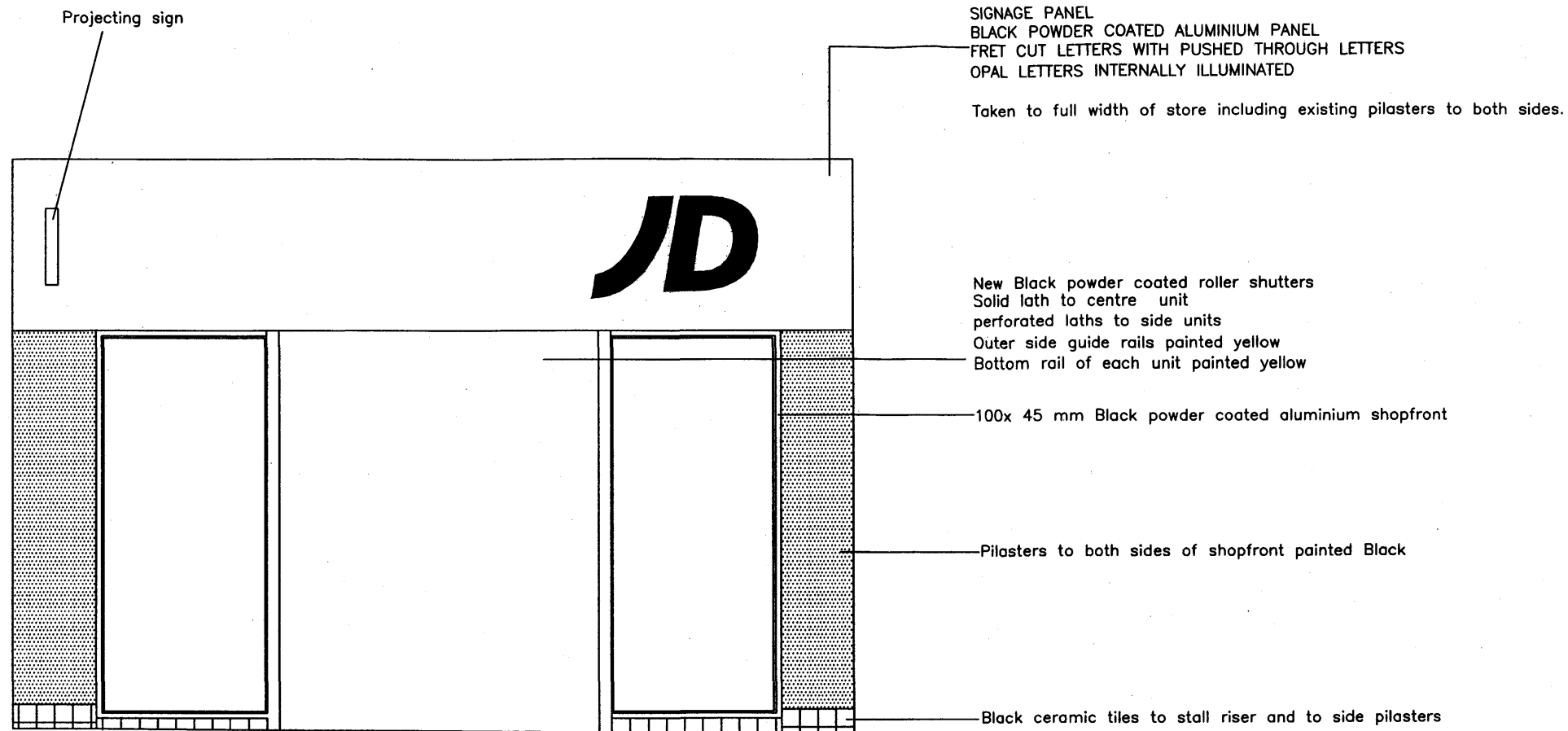
Proposed Elevation
