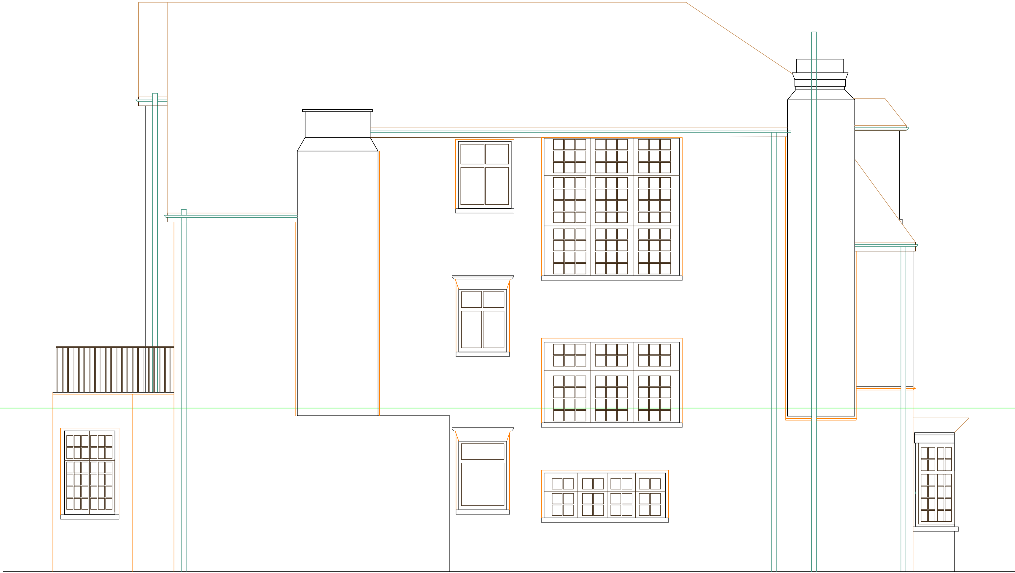
Existing Left Side Elevation
