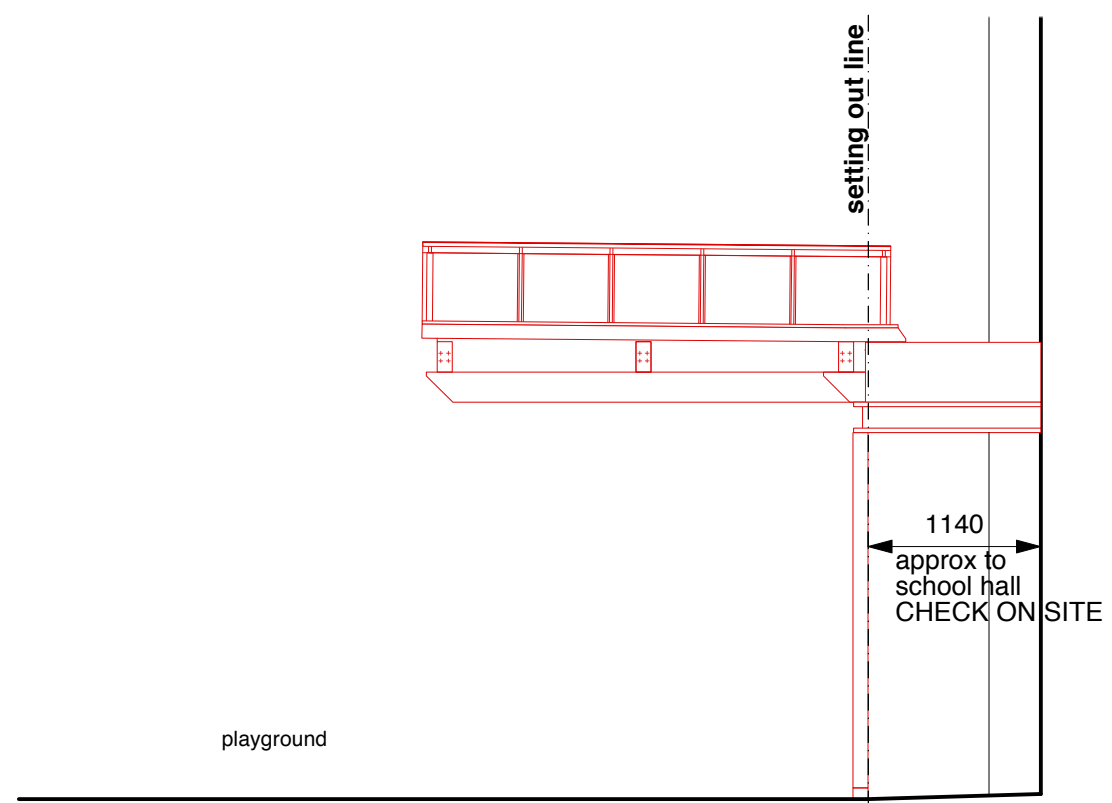
SIDE ELEVATION
