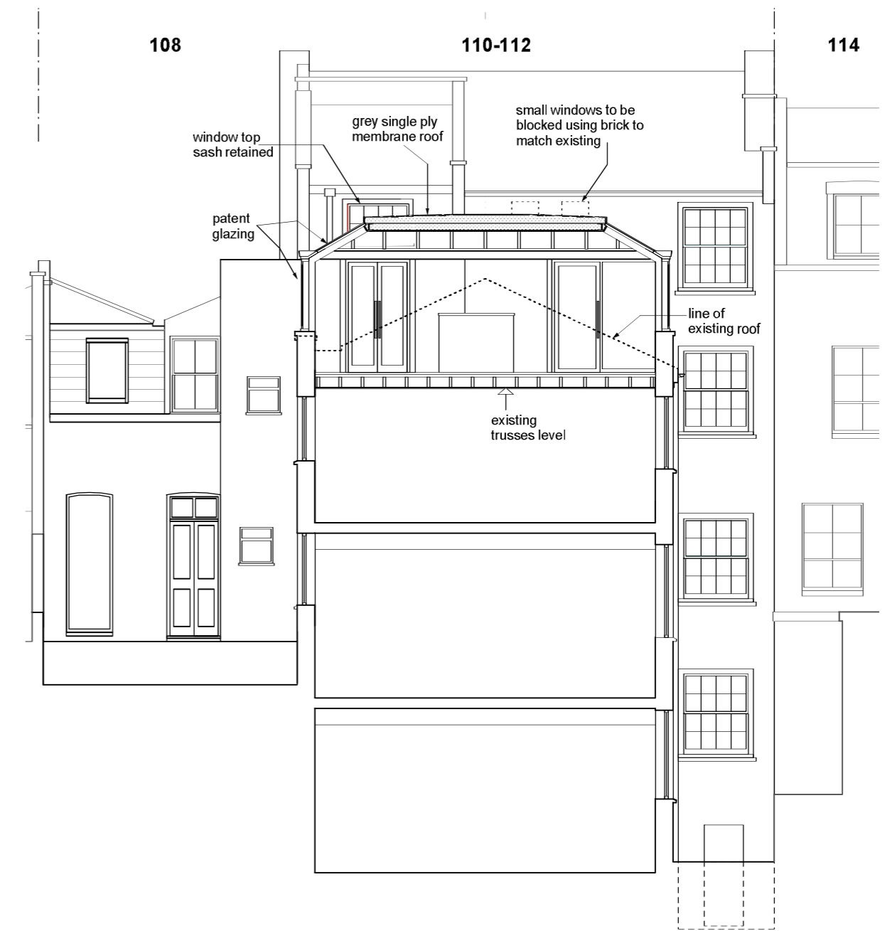
SECTION 5-5 1:100
