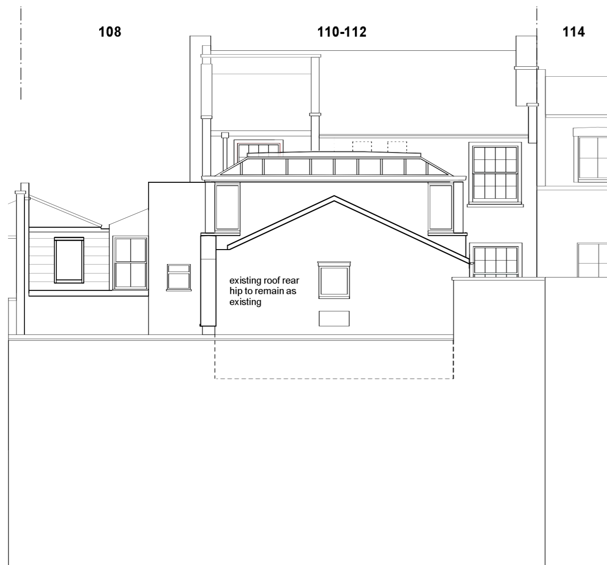
REAR ELEVATION 1:100
