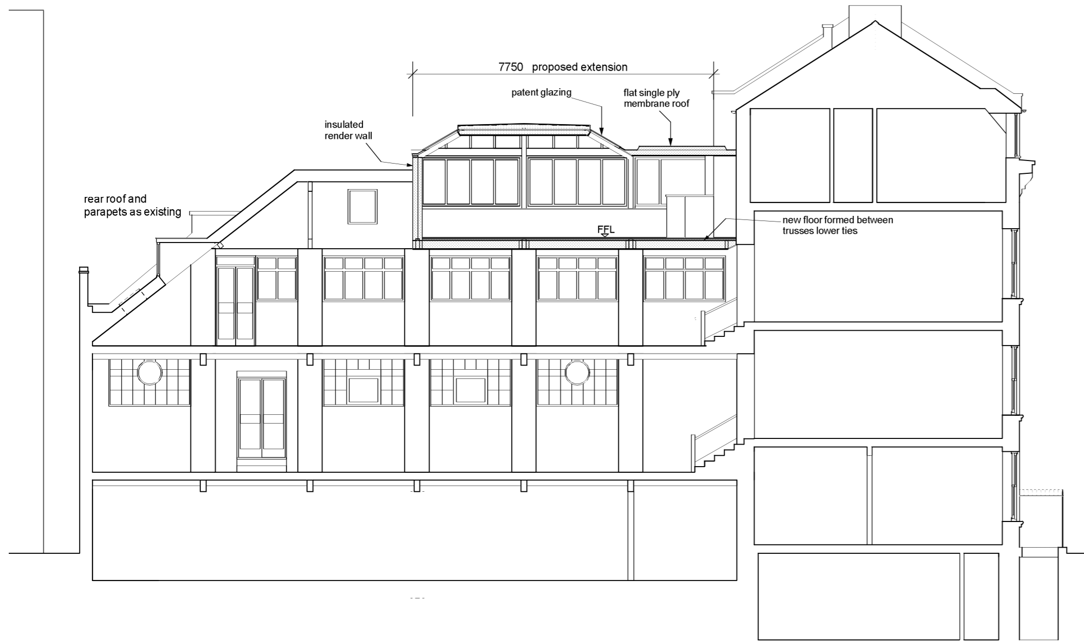
SECTION 4-4 1:100
