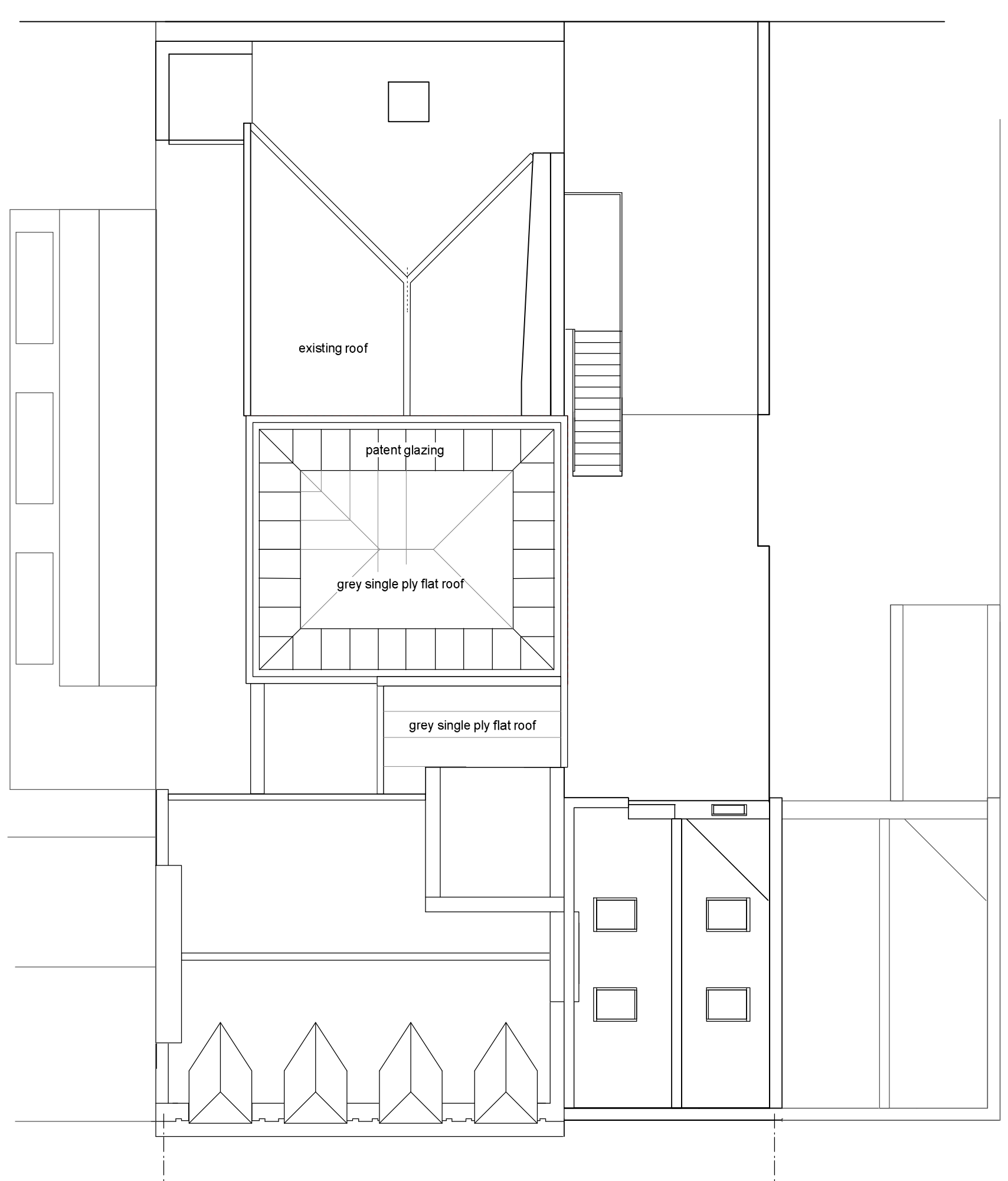
ROOF PLAN
