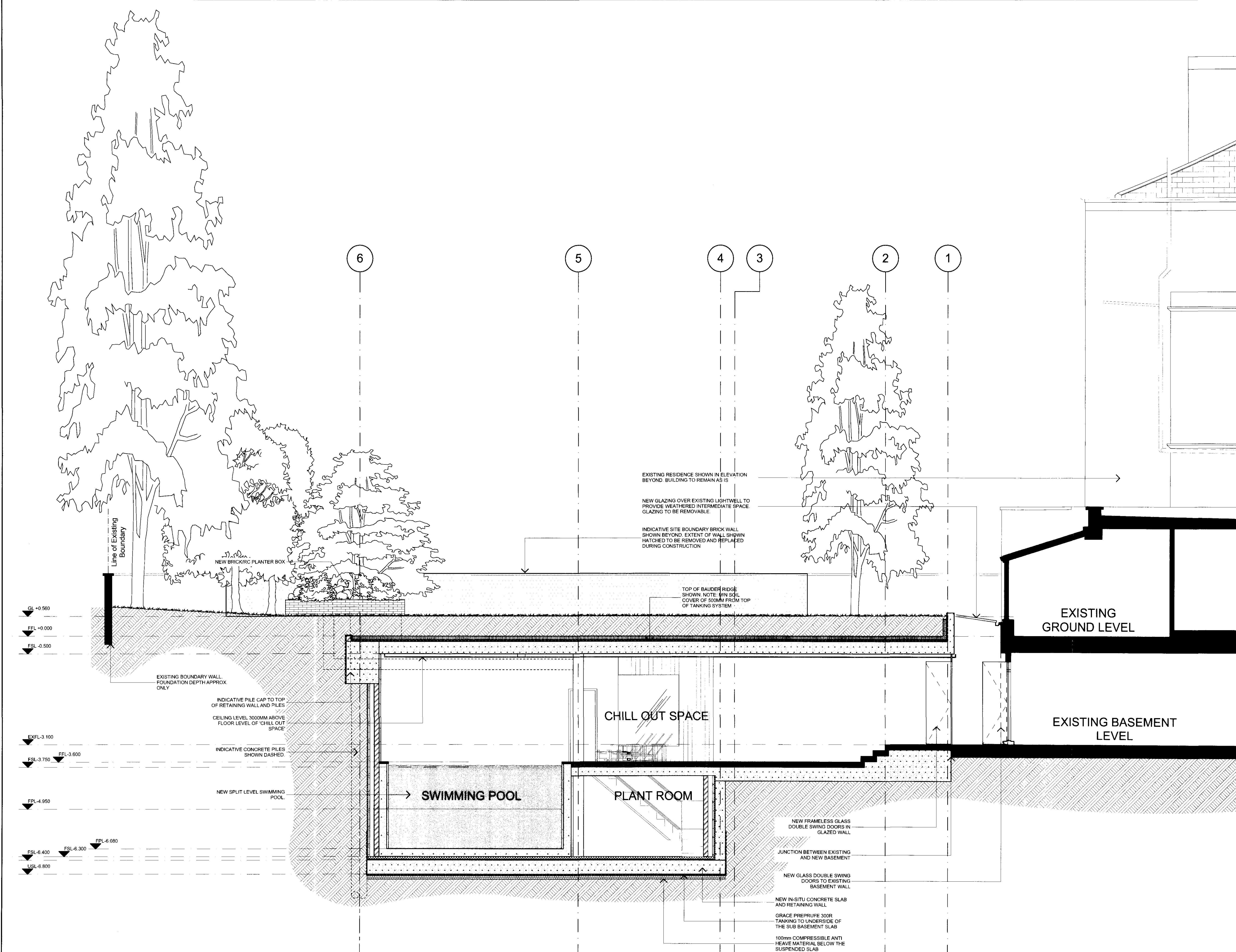
SCALE 1:100 at A3 2 PROPOSED SECTION B - LONGITUDINAL
