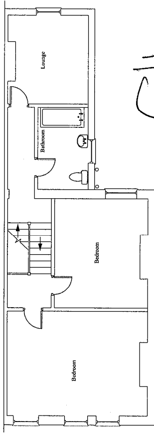
Existing Second Floor Plan
