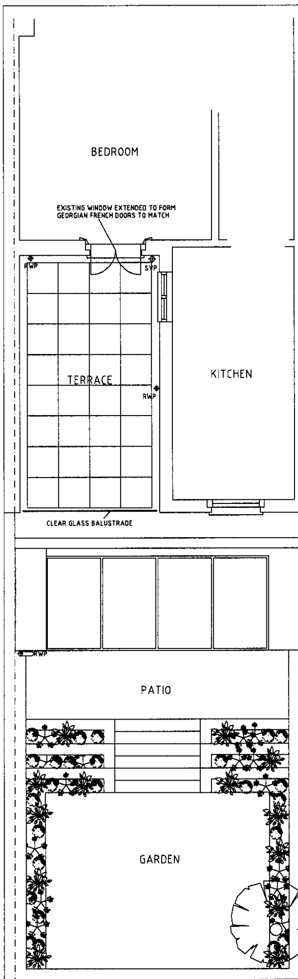
UPPER GROUND FLOOR PLAN
