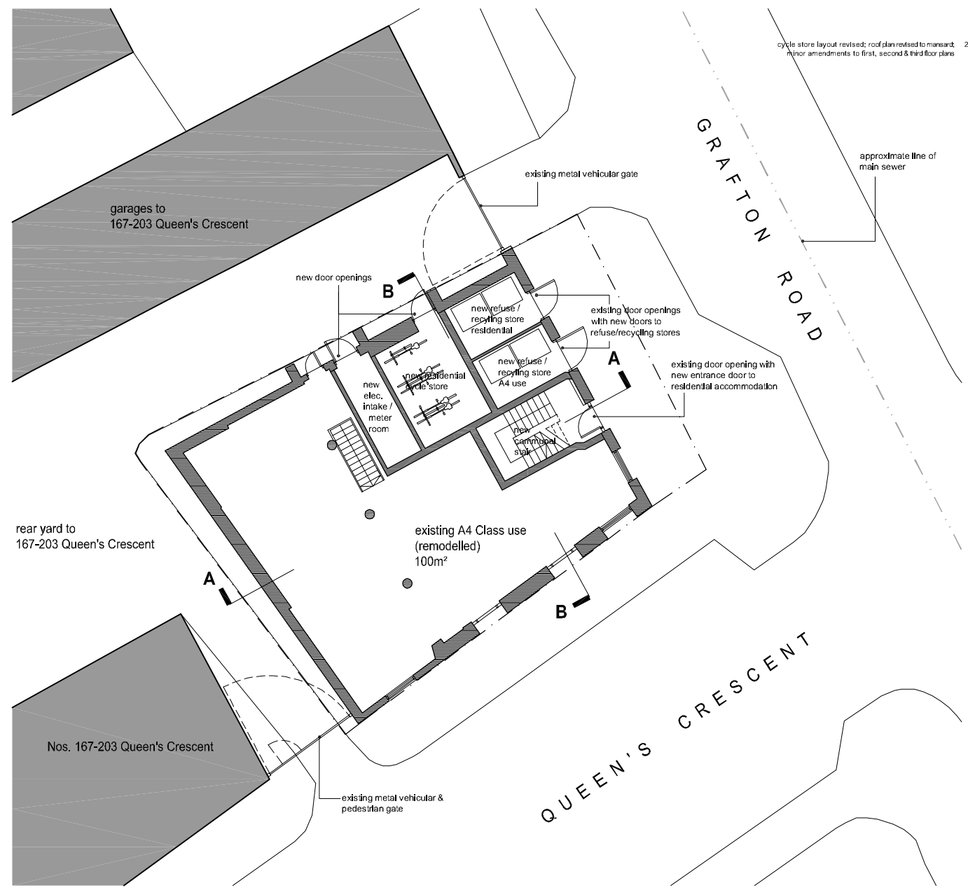
ground floor plan and site layout
