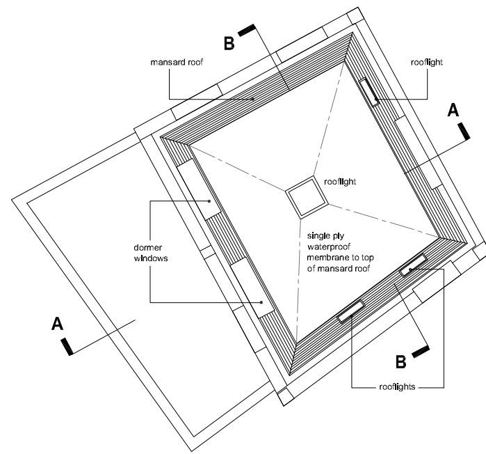
roof plan
