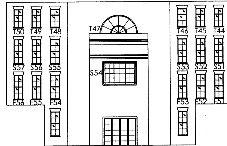
WEST COURTYARD ELEVATION ELEVATION
