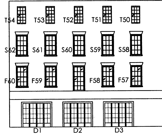
SOUTH COURTYARD ELEVATION
