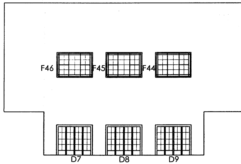
EAST COURTYARD ELEVATION
