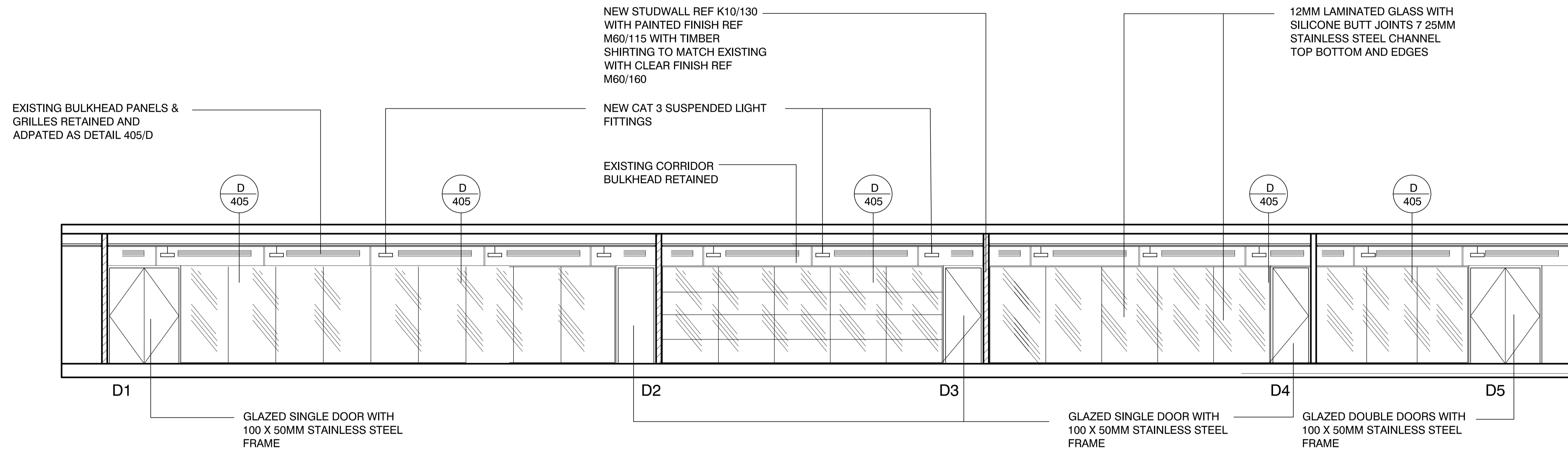
CORRIDOR ELEVATION
