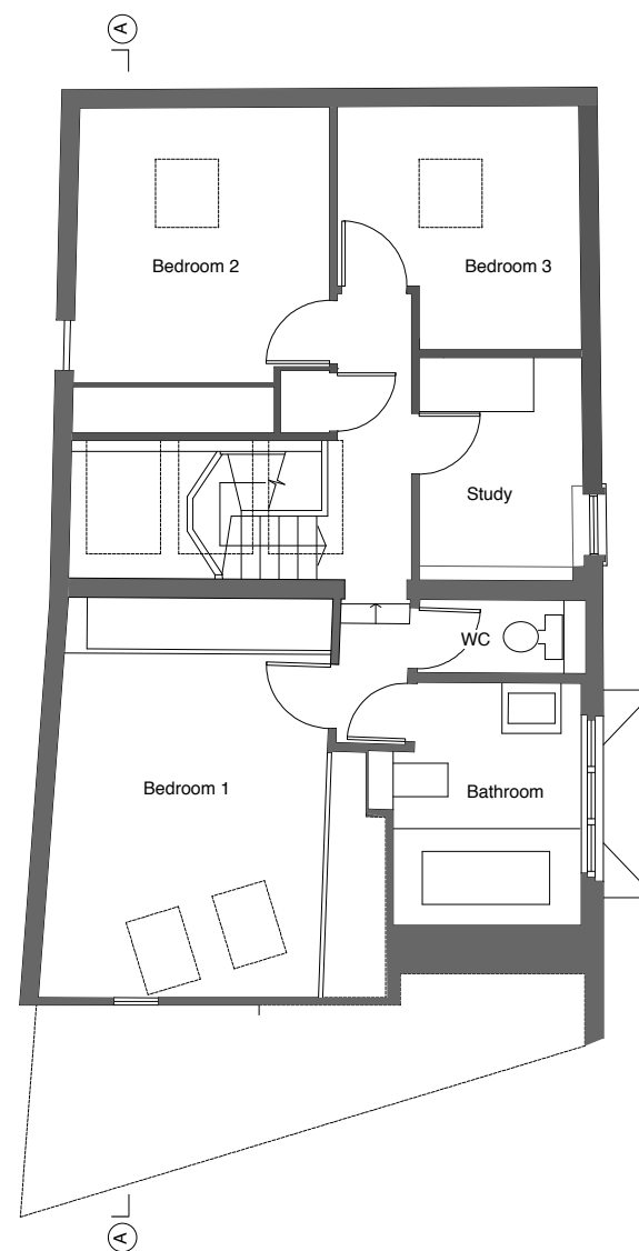
First Floor Plan Existing
