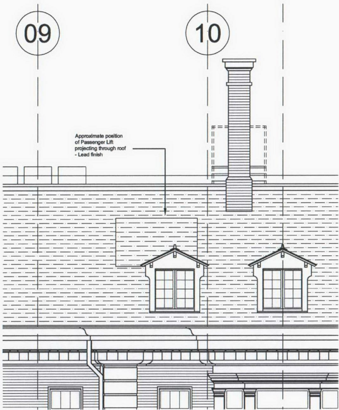
Elevation - Passenger Lift
