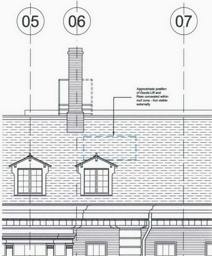
Elevation - Goods Lift
