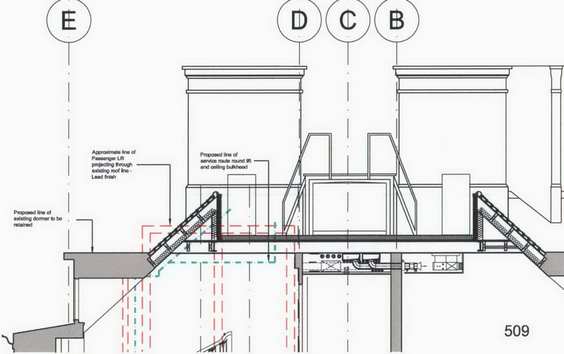
Proposed Passenger Lift and relationship to existing roof profile
