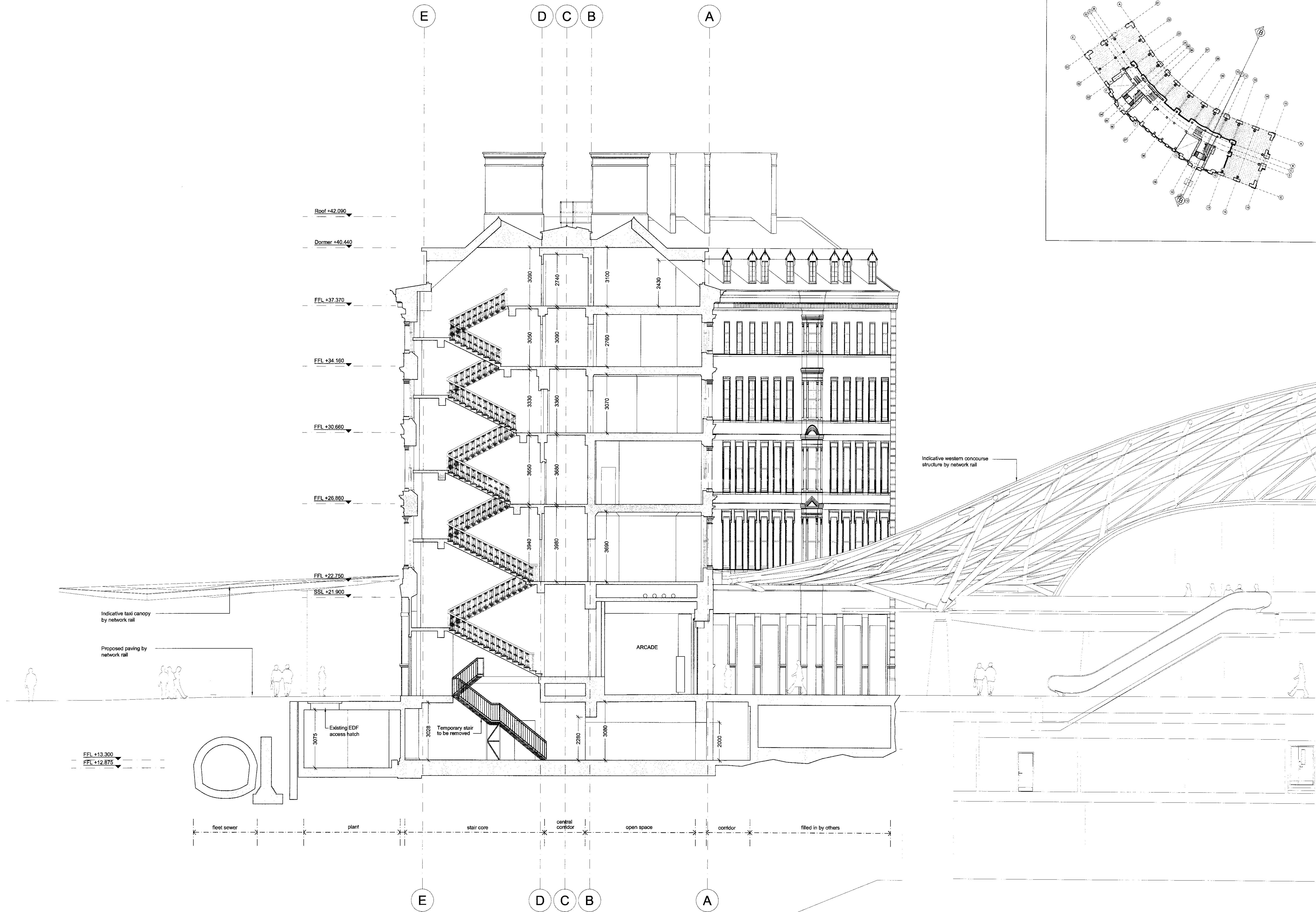
Section BB Scale 1:100 @ A1 (1:200 @ A3) 0 1000 2000 3000 4000 5000 6000 7000 8000 9000 10 000 SCALE BAR (1000 = 1M)
