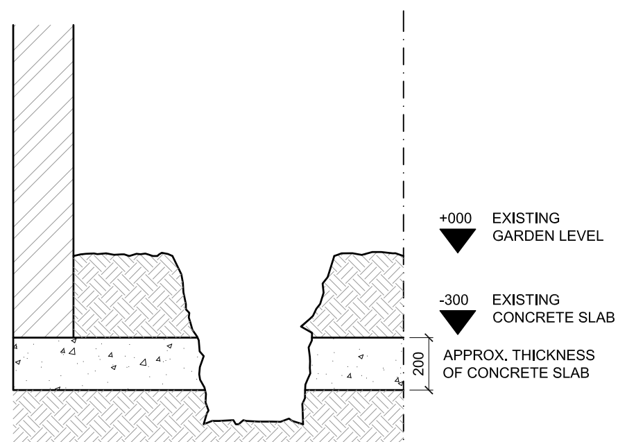
EXISTING SECTION B-B SCLAE 1:20
