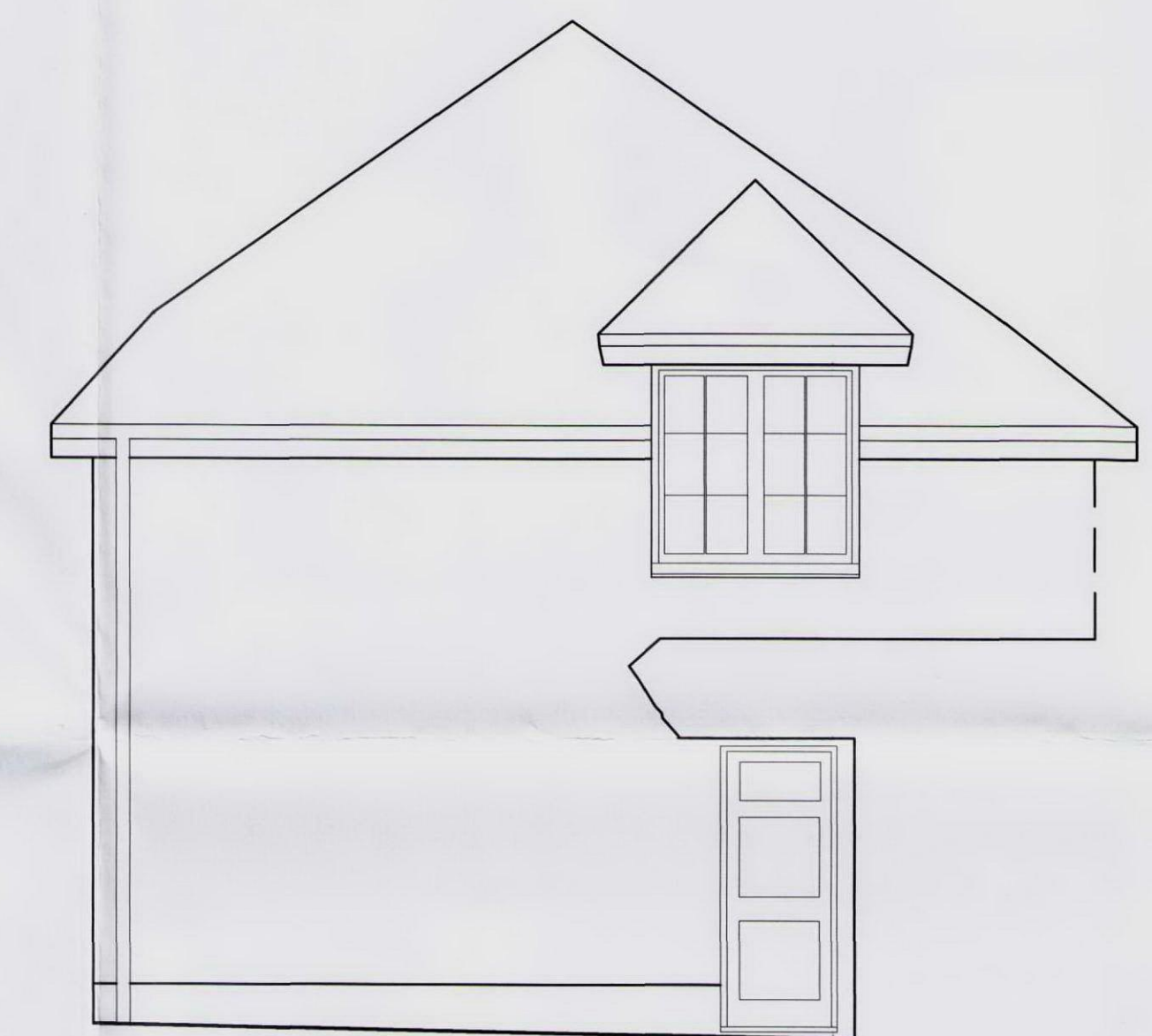
Existing South Garage Elevation
