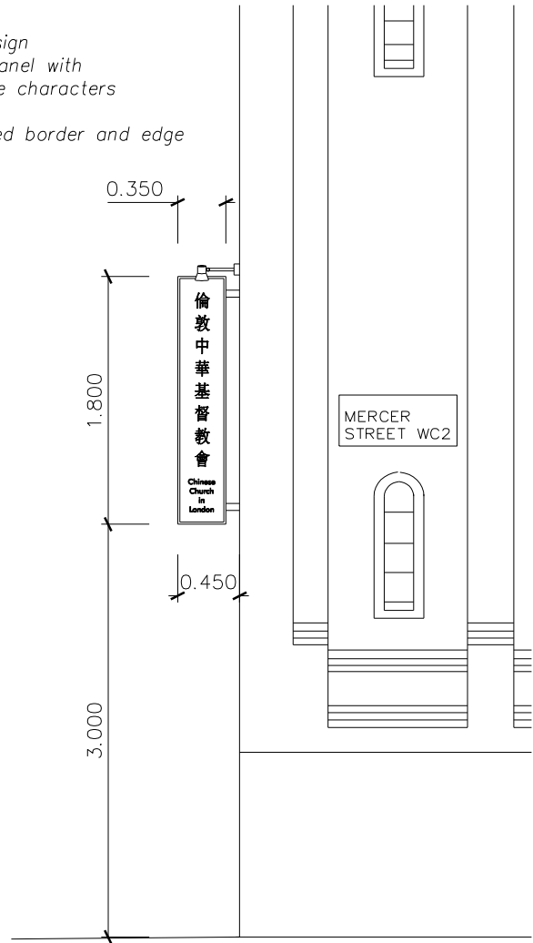
MERCER STREET ELEVATION
