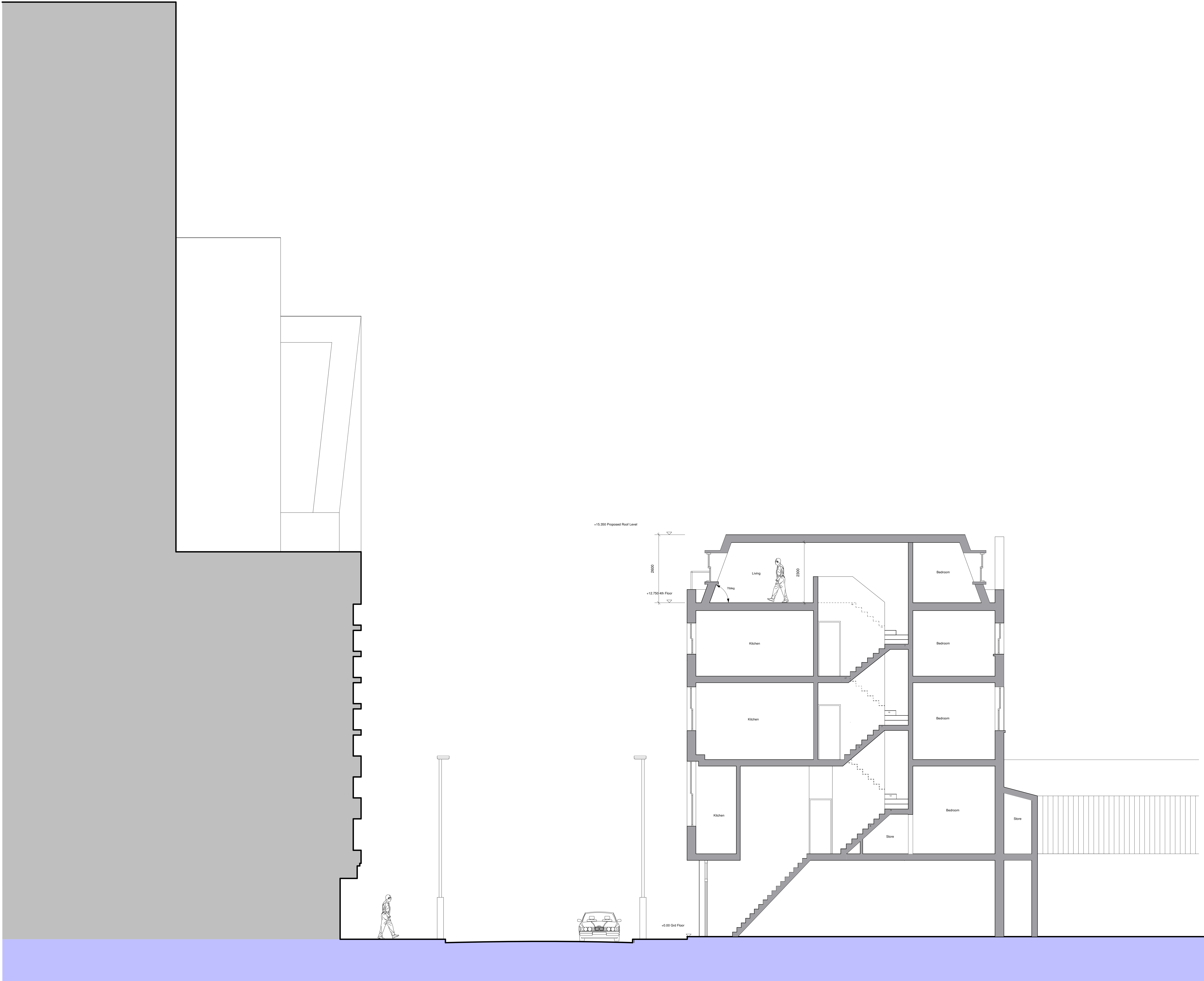
Proposed SECTION A-A (SCHEME A)
