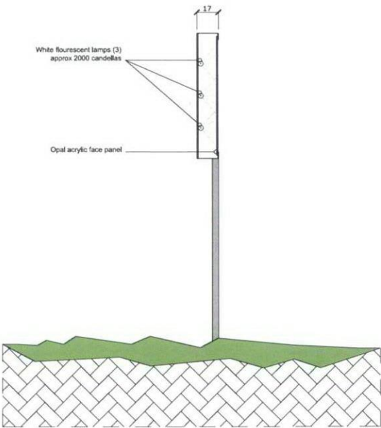
SECTION AA - ILLUMINATED SIGN
