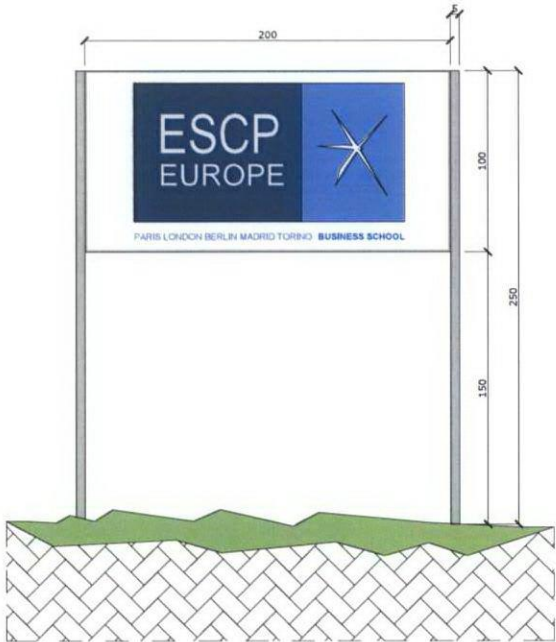
ELEVATION - ILLUMINATED SIGN
