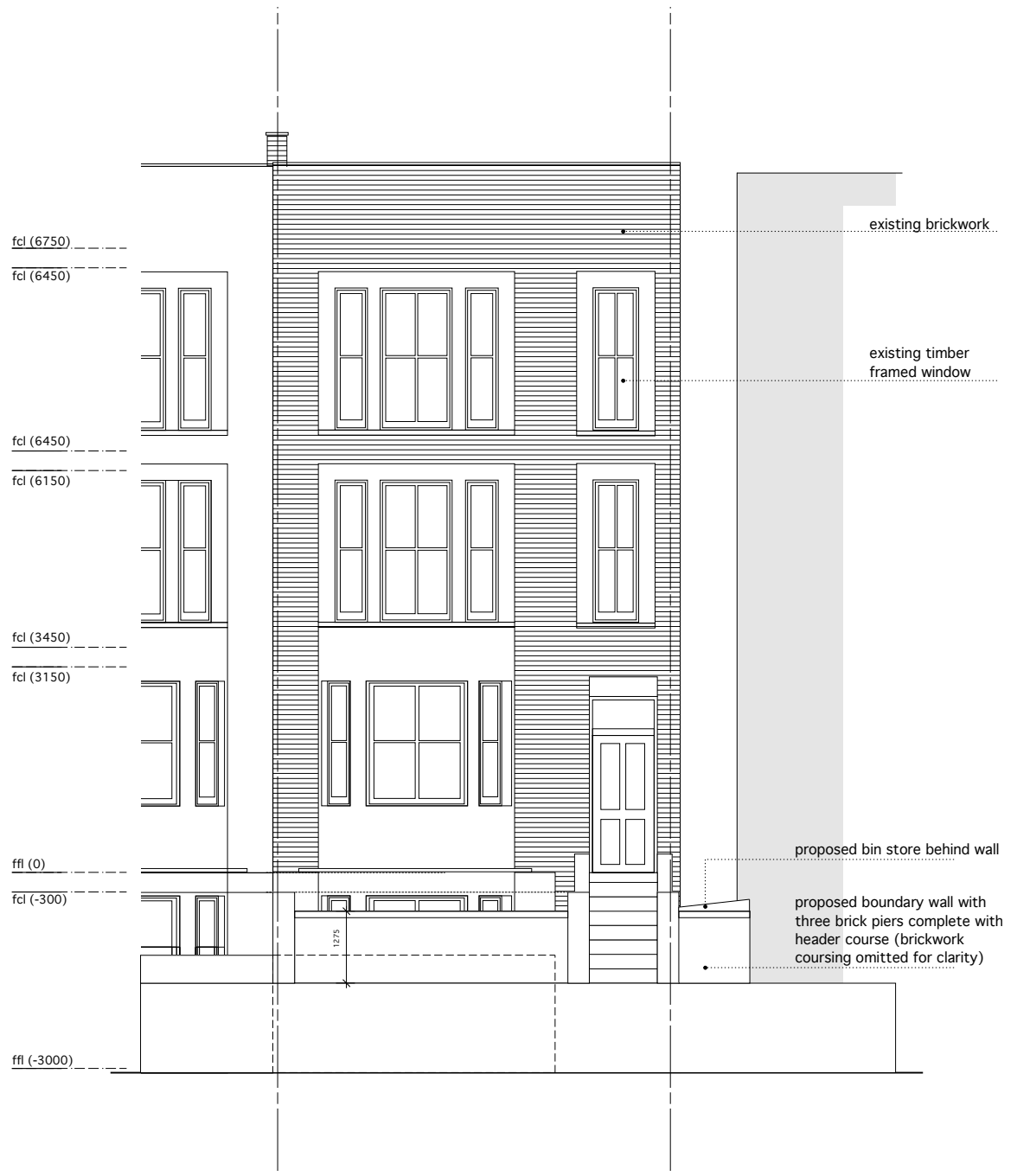
front elevation
