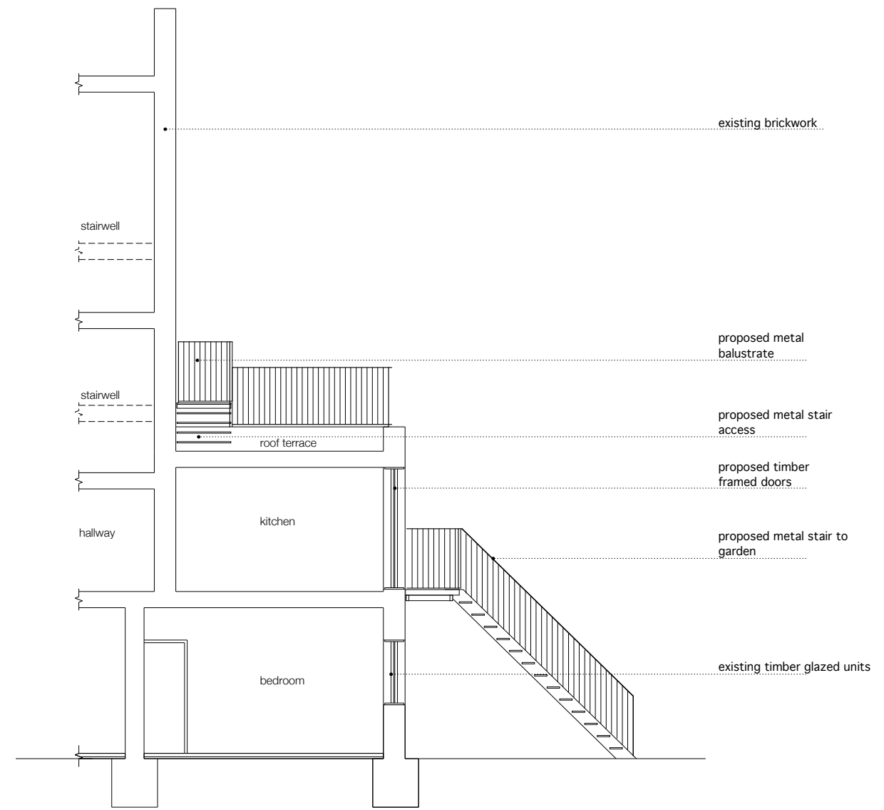
Section 2-2
