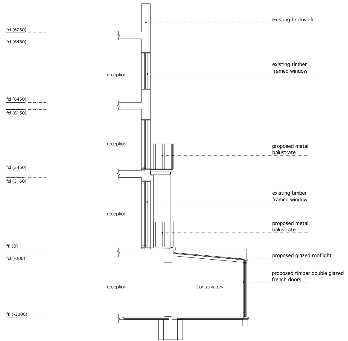
Section 1-1
