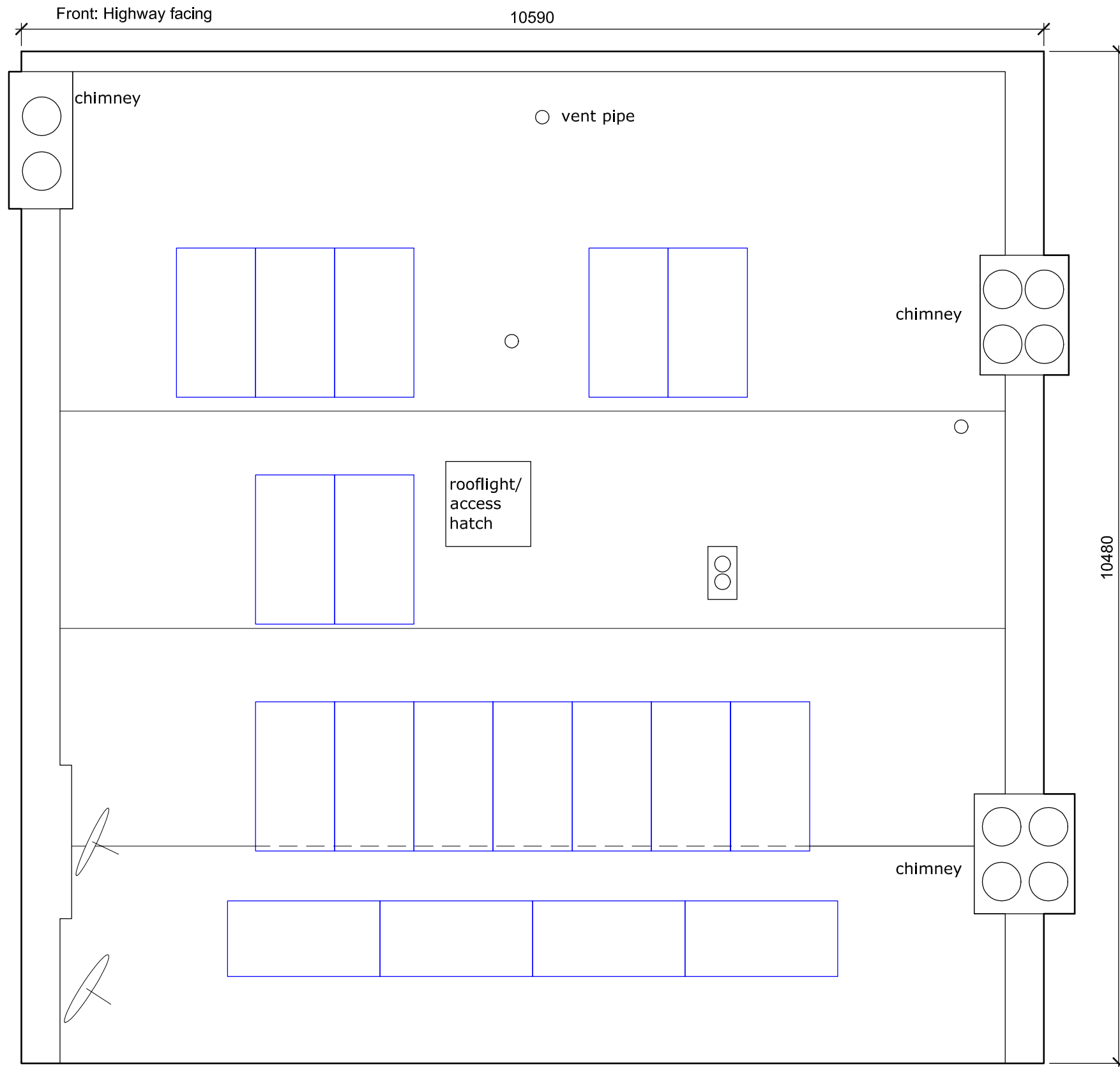
Solar PV installation on the upper roof: 3.87 kWp PV array comprised of 18 Sanyo hybrid 215W panels (see data sheet)
