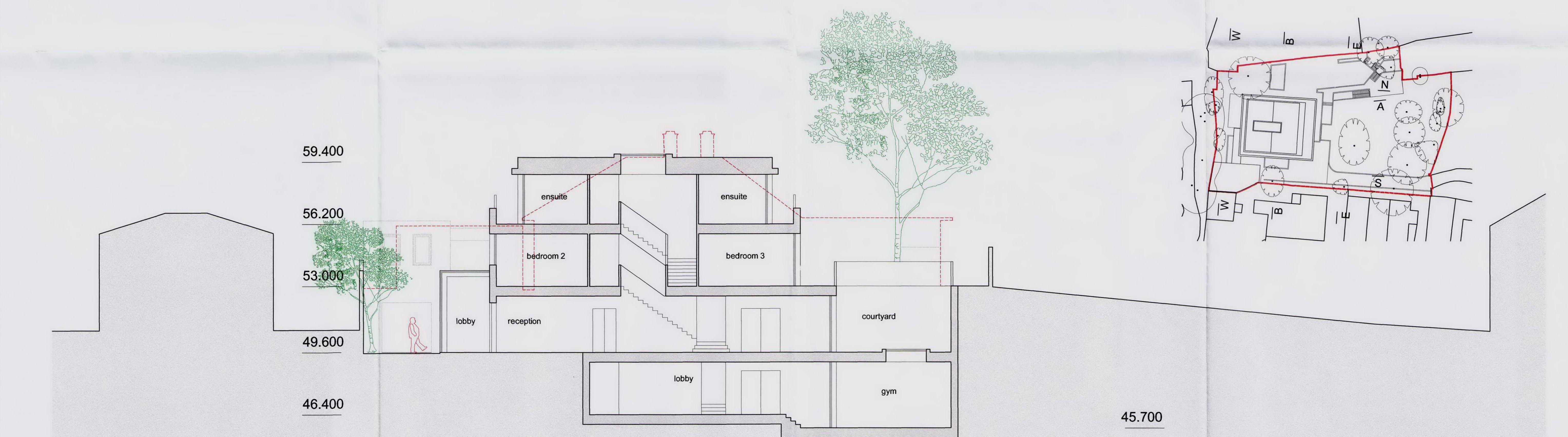
Proposed Section B:B
