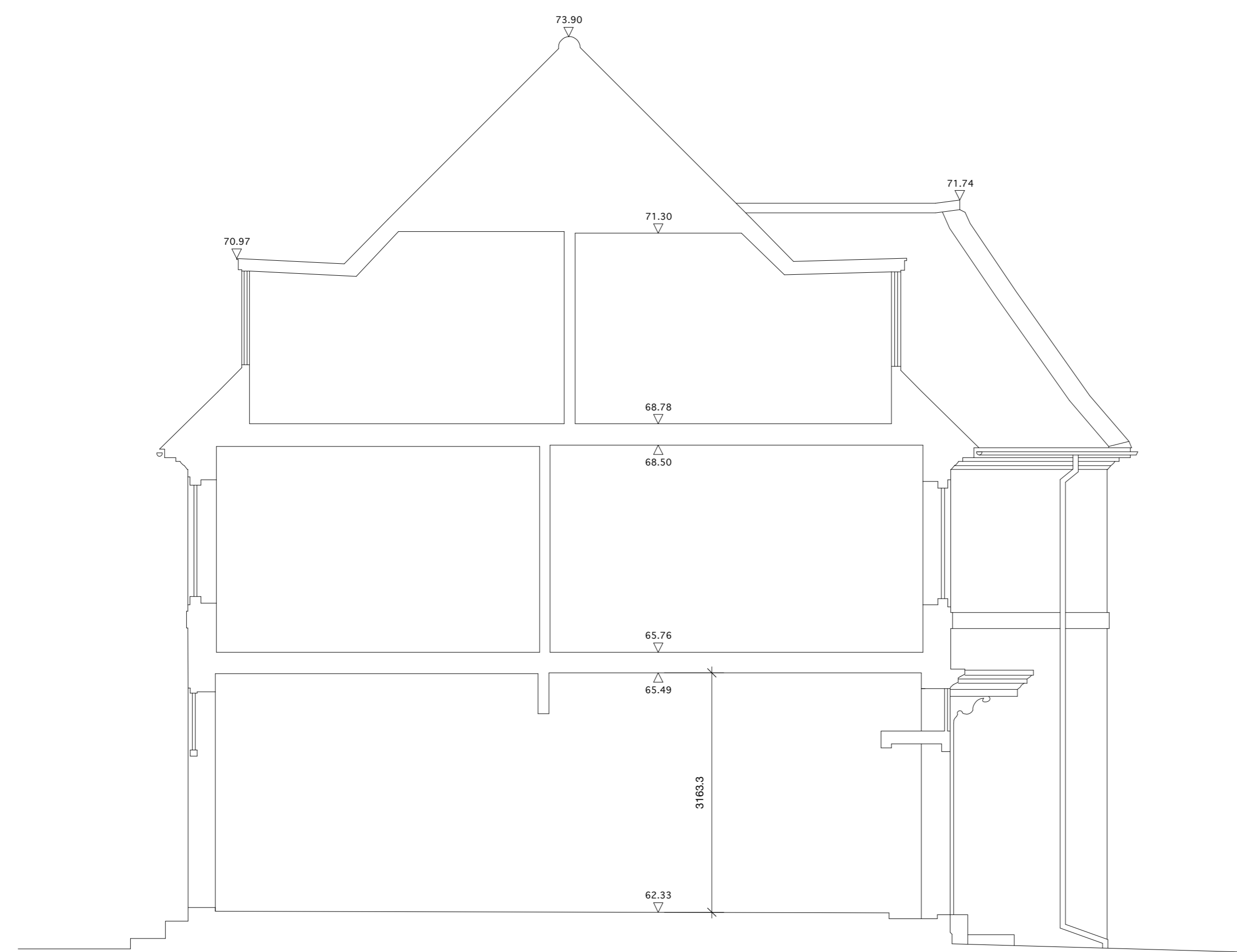
datum 60.00m Section 1
